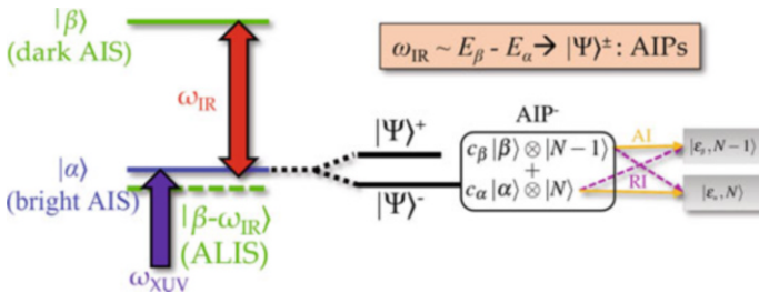
Fig. 3 Schematic representation of AIP formation and subsequent decay pathways. Near resonance, the degeneracy of between a bright ( |\alpha\rangle ) AIS and an ALIS ( |\beta - \omega_{IR}\rangle ) leads to AIP multiplets, which then decay through autoionization and radiative ionization. Destructive interference between these pathways can lead to stabilization of the atom against ionization
