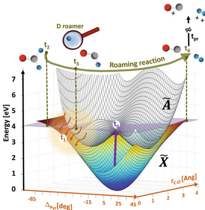
Fig. 1 Schematic of roaming dynamics in D_2CO visualized for two coordinate systems; the orange axis correspond to relevant vibrational modes, the green curved line shows the roaming reaction coordinate. A pump pulse (purple arrow, 304 nm) excites the \tilde{A} state at time t_0 to the purple energy level. Because of vibronic coupling of the out-of-plane bending (pyramidization) and the C–O stretching mode with hot vibrational states of the ground state, a nonradiative population transfer is initiated at t_1 . Once on the hot ground state, three reaction types can occur: D_2 + CO molecular dissociation, D + DCO radical dissociation, and roaming, each following its own reaction potential that is not explicitly shown here. Corresponding exemplary molecular structures for three subsequent times are given along the roaming reaction coordinate (green curved line). Excited molecules experience D_2 vibrations ( t_2 ), which lead to one deuteron roaming around the remaining DCO fragment at large interatomic distances ( t_3 ). Eventually, the roamer D abstracts the bound deuteron and together they leave the CO fragment, which leads to D_2 formation and abstraction ( t_4 ). Note that t_1 to t_4 do not correspond to specific absolute times but rather indicate the order of these steps within a statistical process. A strong NIR pulse (800 nm, \sim 8 fs duration, black arrow) probes the molecular structure at variable time delays ( t_{pr} ). (Figure reprint with permission from Ref. [3])
