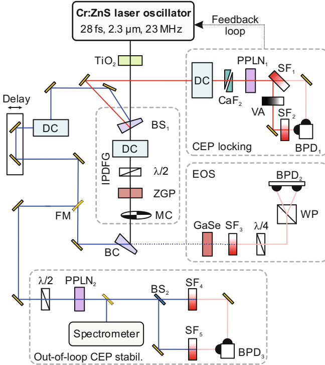
Fig. 1 Schematic of the experimental setup. The output pulses of the Cr:ZnS laser oscillator are spectrally broadened in a 0.5-mm-thick TiO 2 plate and subsequently split into three individual channels by using a wedged beam splitter (BS 1 ): the transmitted beam is used for intrapulse difference-frequency generation (IPDFG), the primary wedge reflection (blue line) acts as a gate pulse for electro-optic sampling (EOS) and the secondary wedge reflection (red line) is used for carrier-envelope-phase (CEP) locking. DC dispersion compensation unit, \lambda/2 half-wave plate, \lambda/4 quarter-wave plate, MC mechanical chopper, BC beam combiner, SF 1-5 spectral bandpass filters, BPD 1-3 balanced photodetectors, WP Wollaston prism, BS 1-2 beam splitters, PPLN 1-2 periodically poled lithium niobate crystals, VA variable attenuator, CaF 2 Calcium Fluoride, FM flip mirror
