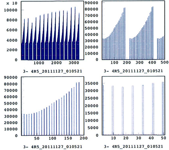
Figure 7: Bunch by bunch luminosity for a Pb store.
