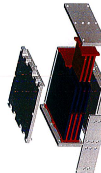
Figure 3: Exploded view of the sensor, showing the ceramic housing and the copper structure segmented in four quadrants and with six gaps.
