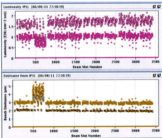
Figure 6: The luminosity and emittance taken on August 6, 2011. On the x-axis is the bunch number.
