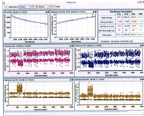
Figure 4: The BRAN operator interface.
