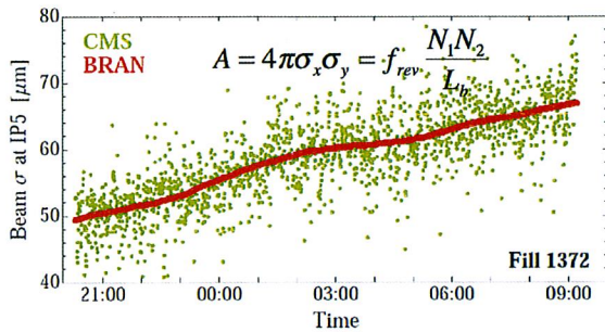
Figure 5: Emittance growth in Fill 1372.
