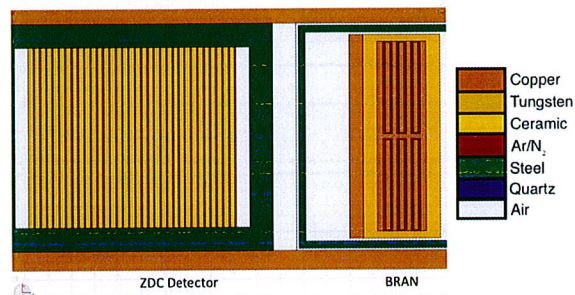
Figure 2: FLUKA model of a BRAN unit installed in the TAN slot behind the ZDC detector (in the 2011 run).
