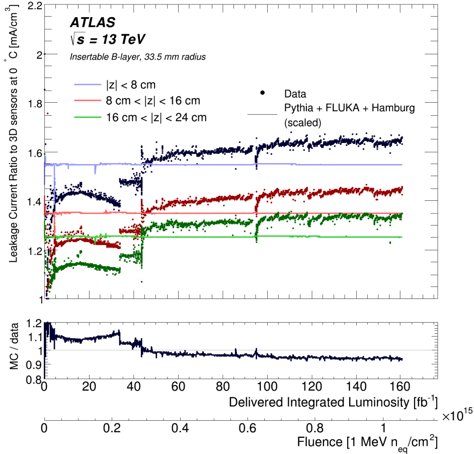
Figure 5: The measured and predicted leakage currents on the Insertable B -layer, both normalized to 0\text{ }^\circ\text{C} , divided by the currents in the 3D modules at 24 < |z| < 32\text{ cm} . The other three module groups represent |z| < 8\text{ cm} , 8 < |z| < 16\text{ cm} , and 16 < |z| < 24\text{ cm} . The A and C sides of the detector ( z > 0 and z < 0 ) are consistent with each other and averaged. The dominant time-independent uncertainty of 10% is not included to avoid overlapping bands. The prediction is based on the thermal history of the modules combined with the Hamburg Model for modelling changes in the leakage current and PYTHIA + FLUKA for simulating the overall fluence. For all four predictions, the overall scale normalization is based on a fit to the data across the entire range. Normalization factors are determined per |z| region. The lower panel shows the ratio of the prediction to the data for the innermost module group. Similar MC/data trends are observed for the other three |z| regions. For illustration, the fluence is shown as a lower horizontal axis using the nominal luminosity-to-fluence from simulation at |z| = 0 .
