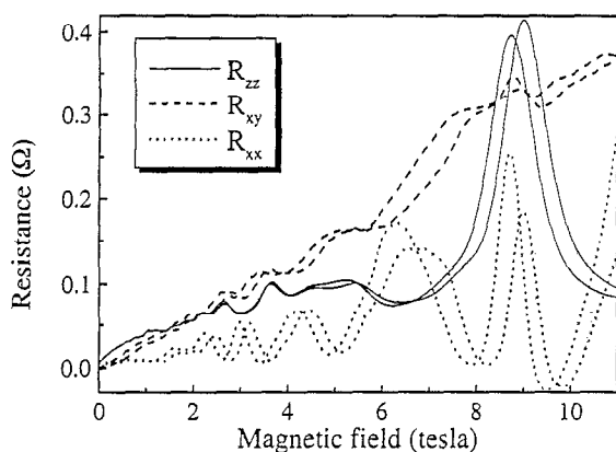
Fig. 3. Temperature dependence of R_{zz} (sample #2). The 100 mK R_{xx} and R_{xy} data from Fig. 2 is included for comparison.
