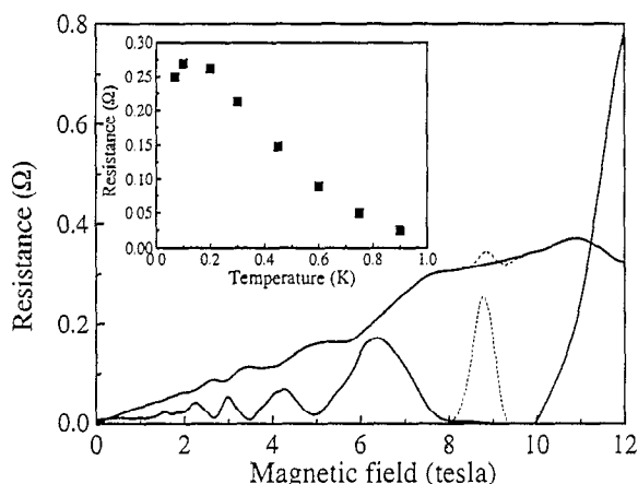
Fig. 4. Corrected R_{xy} and R_{xx} data for sample #1 at 100 mK. The inset shows the temperature dependence of the resistance peak attributed to R_{zz} at 9 T (dashed line in main part of figure).
