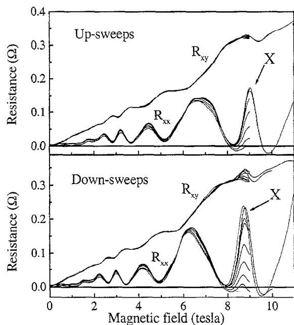
Fig. 2. Temperature dependence of R_{xx} and R_{xy} below 1 K (sample #1). The strongly temperature dependent features are artifacts (see text). The data were taken at more-or-less evenly spaced intervals in temperature from 900 mK to 70 mK; the lowest temperature data have the largest R_{xx} maxima.
