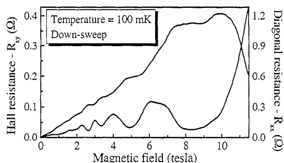
Fig. 5. R_{xy} and R_{xx} data for sample #3.
