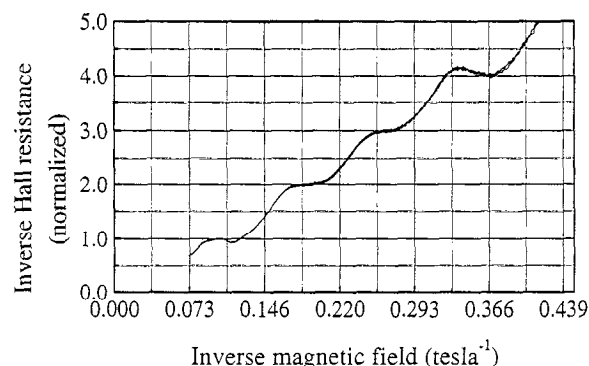
Fig. 6. Hall effect data for sample #4 at 125, 220 and 400 mK (over-laid). R_{xy}^{-1} has been normalized to its value at 9 T in order to demonstrate the excellent quantization.
