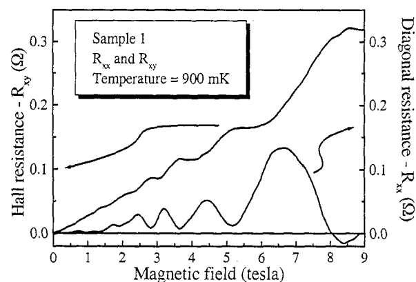
Fig. 1. Representative magnetotransport data for \eta -Mo 4 O 11 .
