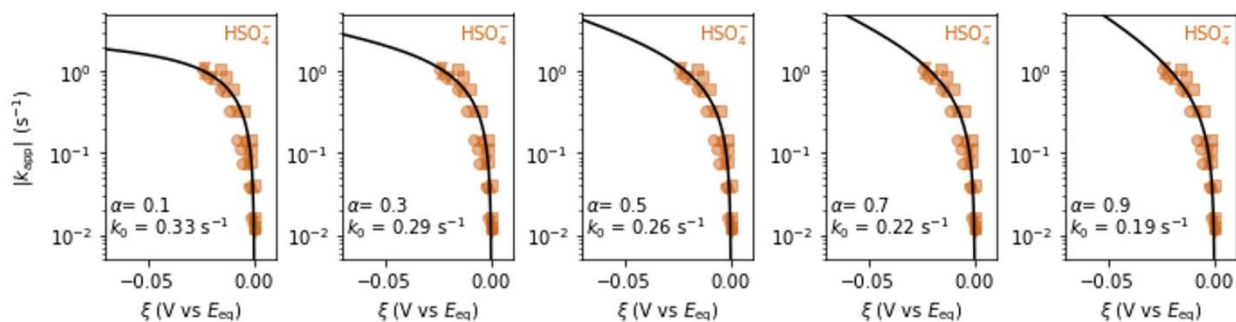
Figure S7: Sensitivity analysis of the parameter \alpha on the calculated k_0 via curve-fitting for for 1 mM \text{Cu}^{2+} dissolved in 10 mM \text{H}_2\text{SO}_4 with rates measured at \theta = 0.05 .
