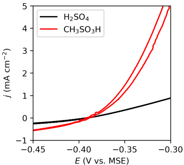
Figure S6: Corrosion behavior for a Cu disk freshly electropolished in \text{H}_3\text{PO}_4(\text{aq}) . The potential was swept in \text{N}_2 -purged \text{H}_2\text{SO}_4(\text{aq}) (black) or \text{CH}_3\text{SO}_3\text{H} (red) at \nu = 5 \text{ mV s}^{-1} at a constant rotation rate of 1600 rpm.
