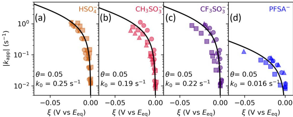
Figure 5. Interfacial Cu transfer apparent interfacial ion transfer rate vs driving force at 5% coverage of Cu on an Au(111) surface in 1 mM CuO in (a) 10 mM \text{H}_2\text{SO}_4 , (b) 10 mM MSA (c) 10 mM TFMSA and (d) 10 meq PFSA - ionomer electrolyte. Data were fit with Equation 4 (solid black line) to calculate k_0 . Independent replicates for freshly cleaned Au(111) electrodes are represented by circles, squares, or triangles.
