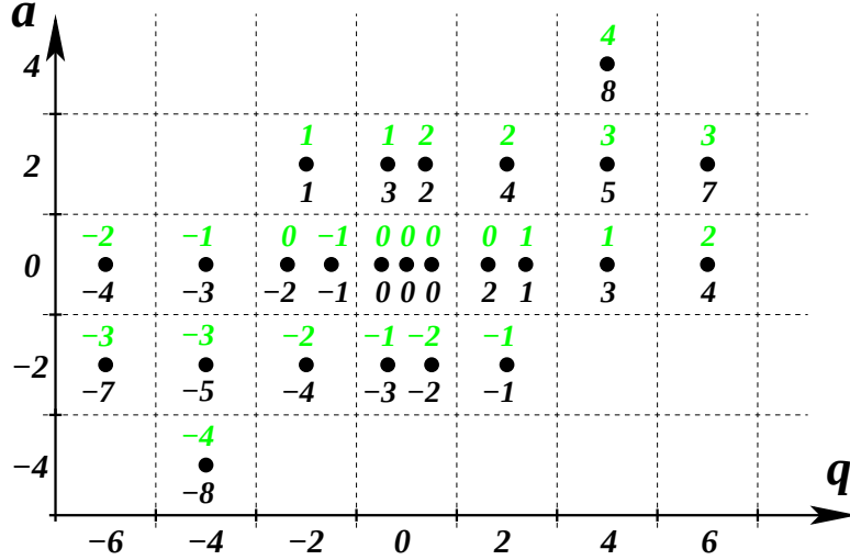
FIGURE 17. The S^2 -colored homology of the figure-eight knot.
