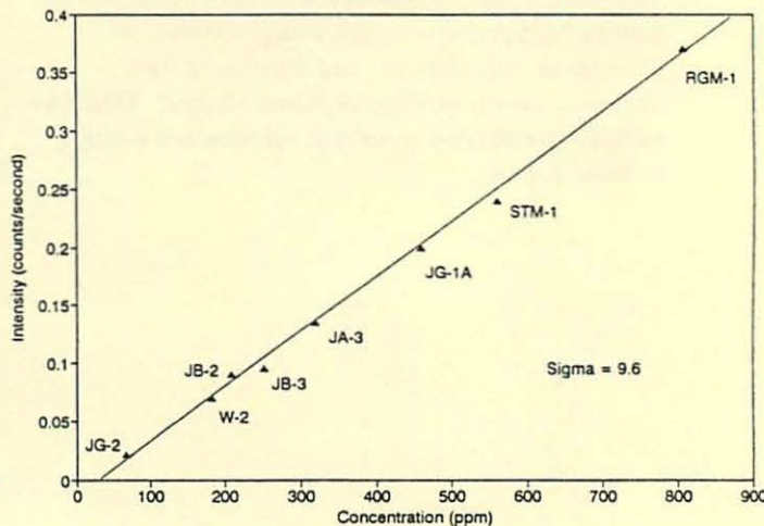
Figure 3. Intensity vs. Concentration: Barium/R2
