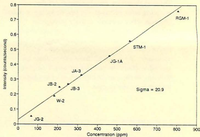
Figure 2. Intensity vs. Concentration: Barium/R1
