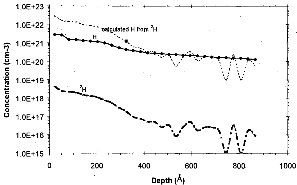
Figure 3.23. Measured ^1\text{H} , ^2\text{H} and calculated ^1\text{H} SIMS depth profiles of a As + Be implanted p-type GaN:Mg film exposed to deuterium plasma at 600°C for 1 hour after annealing at 1500°C for 30s.
