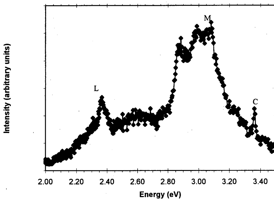
Figure 3.13a. 12K PL spectrum of p-type GaN:Mg implanted with As and Be ( 10^{14} \text{ cm}^{-2} ); annealed at 900^\circ\text{C} for 10 minutes.
