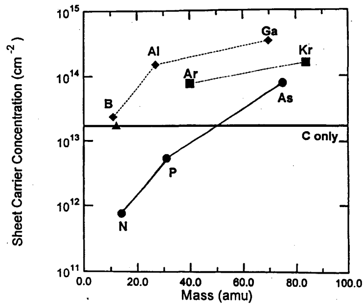
Figure 6. Sheet carrier concentration as a function of the atomic mass of the co-implant species. Samples were annealed at 950°C for 10 s. (Moll et al., 1993)
