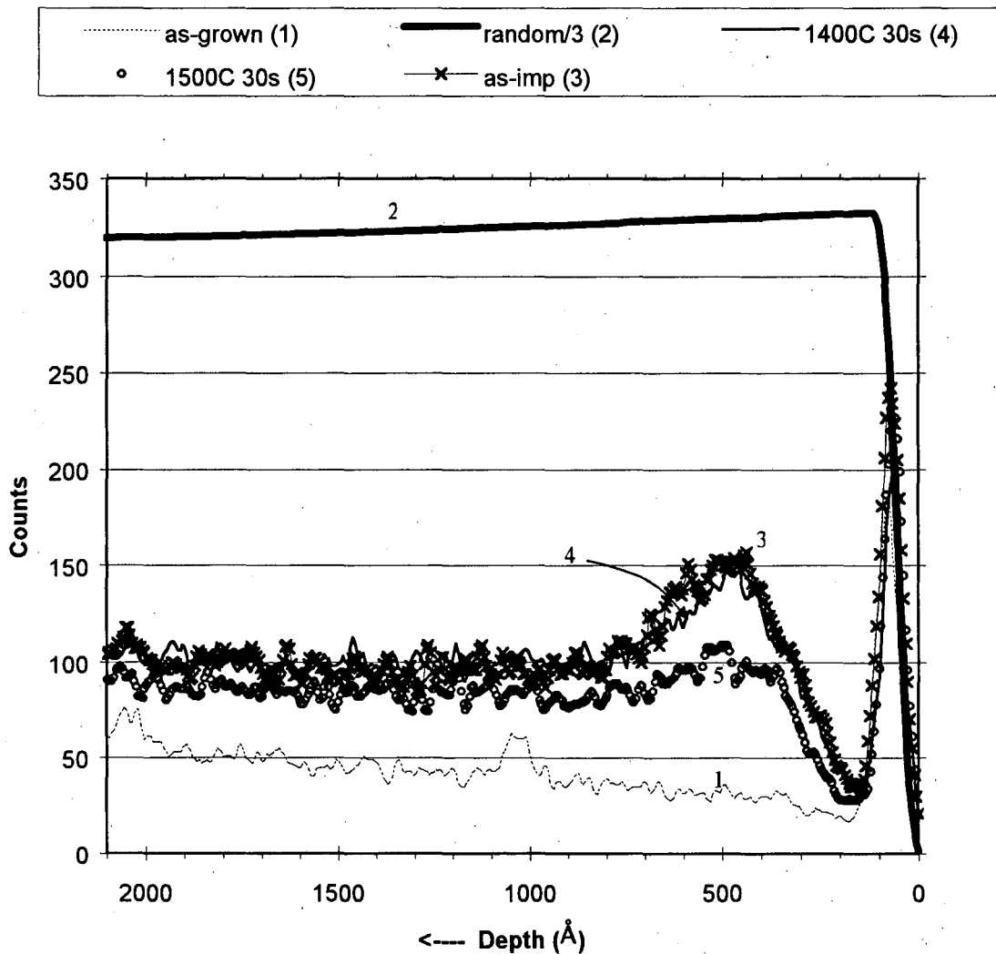
Figure 3.2a. 1.92 MeV \text{He}^+ \langle 0001 \rangle aligned RBS spectra of GaN layers implanted with As ( 10^{15} \text{ cm}^{-2} ) with different annealing treatments.
