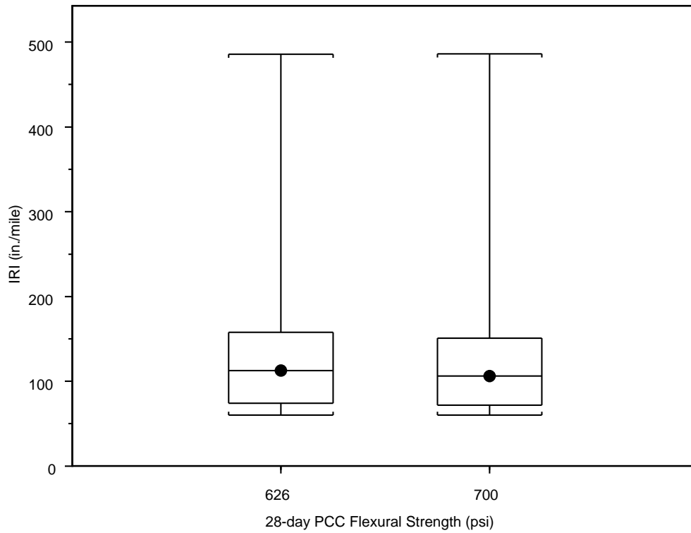
Figure 34. Effect of PCC flexural strength on IRI.
