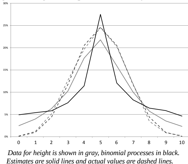
Figure 5: Height vs. Repeated Probability Estimates
