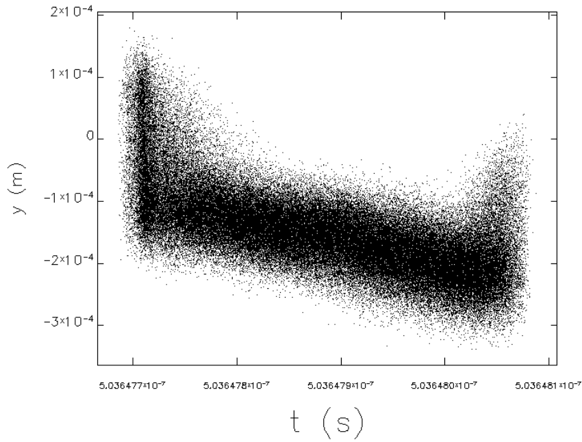
Figure 5-4: FEL input beam vertical distribution along the bunch
