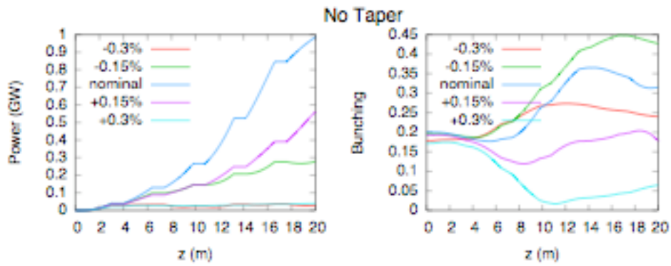
Figure 4-11: Output power and bunching vs. z , for different electron beam energies, no tapering.
