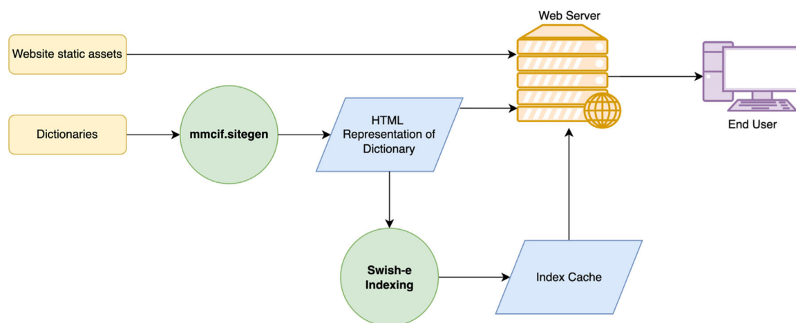
Figure 5. Process flow diagram of producing files for the mmcif.wwpdb.org website. The dictionary ( storedingithub.com/rcsb/mmcif_website_file_assets ) is converted to HTML using the mmcif.sitegen package. These HTML files are combined with the website assets ( github.com/rcsb/mmcif_website ) to serve as the static content of the site. The HTML files produced from the dictionaries are indexed with Swish-e to provide for search capability. Color coding: process inputs (yellow), programs run (identified in green circles), and resulting output files (blue).
