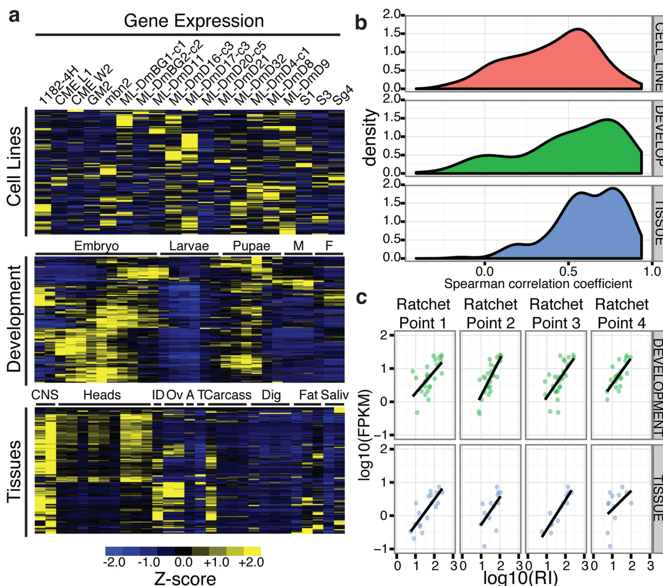
Figure 4. Expression characteristics of recursively spliced Drosophila genes
