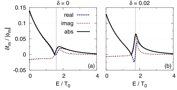
FIG. 1. Eigenfunction for Case 1 (flat density profile), m = 10 , at \psi = 0.5 . (a) No electron dissipation. (b) Finite electron dissipation \delta = 0.02 . A dotted vertical line corresponds to the energy such that the resonance condition \omega = m\omega_d(E) = m\Omega_d E is satisfied.
