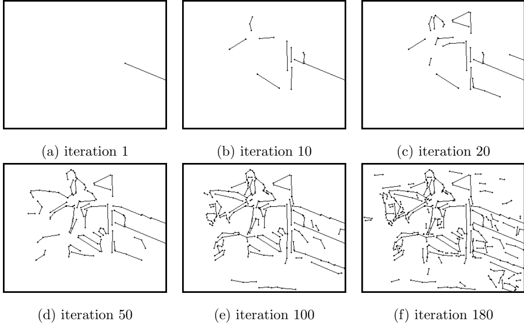
Figure 11: The process of applying operators O_1 and O_2 iteratively for the horse-riding image at iterations of 1, 10, 20, 50, 100, and 180.
