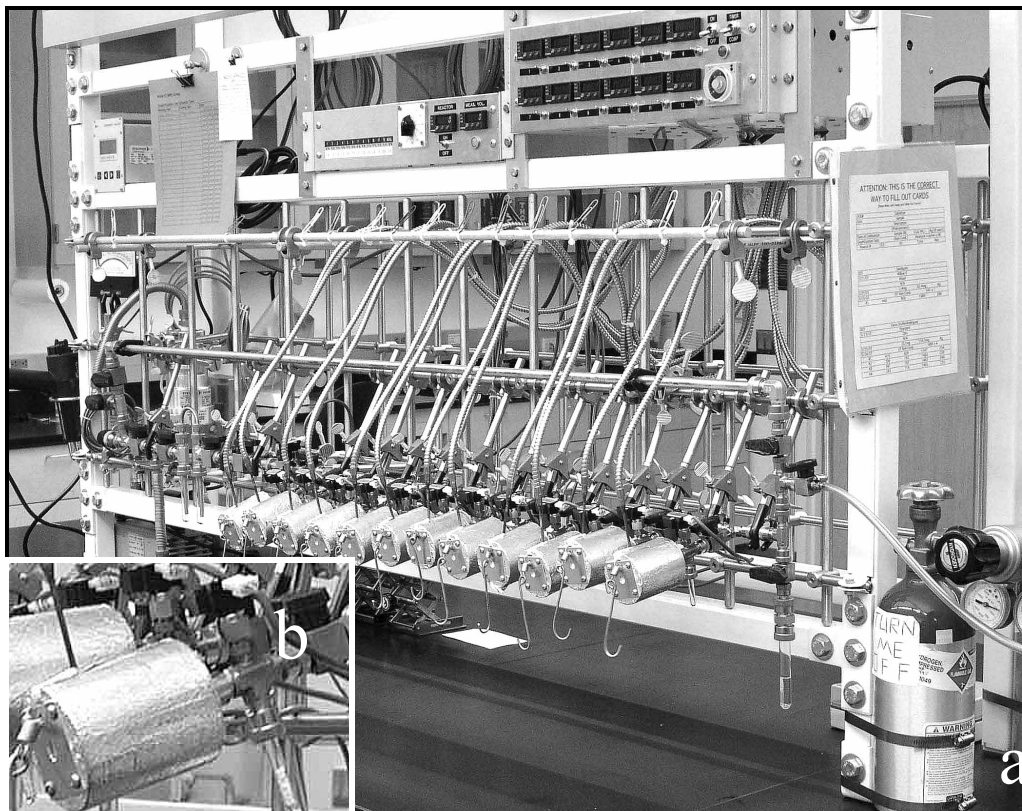
Figure 1 a) Graphitization line for target preparation showing H_2/Fe reduction reactors. Each 12-head graphitization line can produce 24 samples per day. The design is based on graphitization lines from the CAMS/LLNL laboratory. b) Reduction reactor detail showing Mg(ClO_4)_2 in the graphite-reactor.
