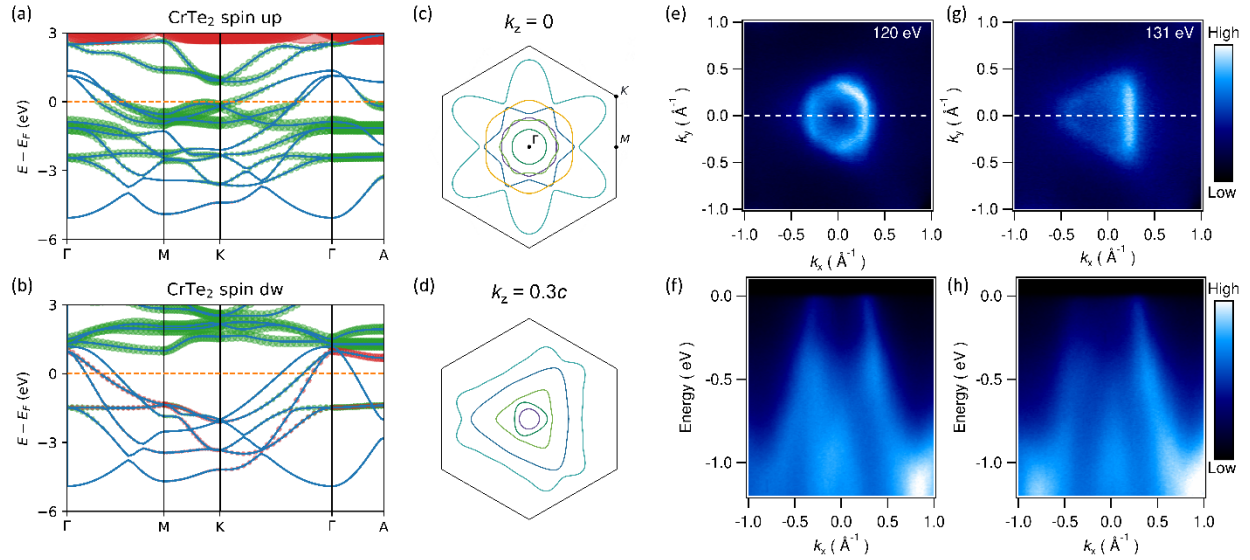
Figure 5 (a)-(b) Calculated spin polarized band structure of CrTe 2 spin up and spin down respectively. Fermi level is highlighted by the orange line. Cr 3 d and Te 5 s , 5 p contribution are shown in green and red, respectively. (c)-(d) Two-dimension slice of the Fermi surface with both spin up and spin down along (001) passing through the \Gamma point and with a distance 0.3c to the \Gamma point, the k_x from \Gamma to M is 0.9 \text{ \AA}^{-1} (e) Experimental Fermi surface plots of Cr 1.21 Te 2 at photon energy of 120 eV. (f) Band dispersions along the high symmetry lines of k_y = 0 of (e). (g) Fermi surface plots of Cr 1.21 Te 2 at photon energy of 131 eV. (h) Band dispersions along the high symmetry lines of k_y = 0 of (g).
