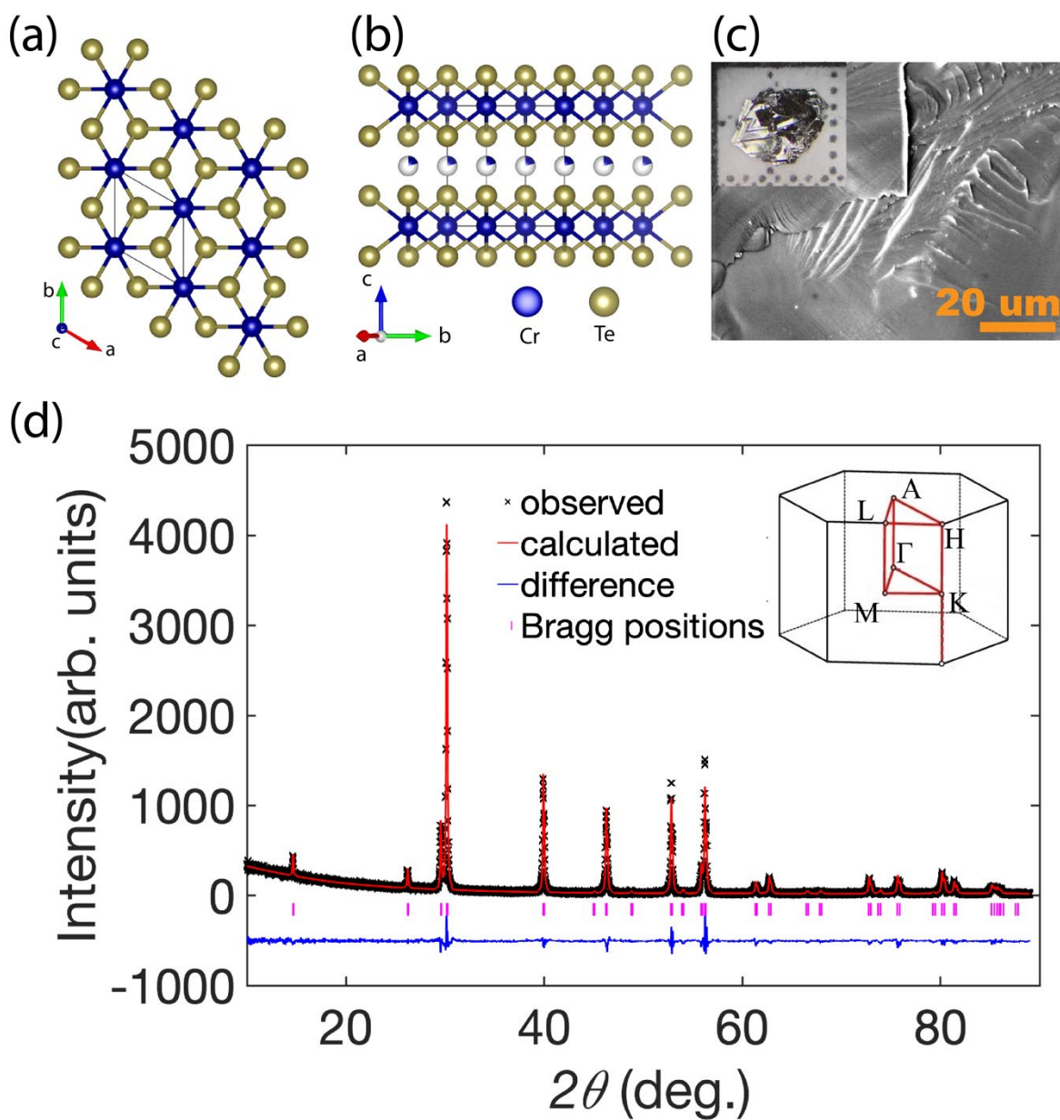
Figure 1 (a, b) Crystal structure of \text{Cr}_{1.21}\text{Te}_2 (top and side views). Grey lines represent a unit cell. (c) SEM image of a \text{Cr}_{1.21}\text{Te}_2 single crystal. Inset: a single crystal of \text{Cr}_{1.21}\text{Te}_2 on a millimeter grid paper. (d) powder x-ray diffraction data of \text{Cr}_{1.21}\text{Te}_2 . Inset shows the Brillouin zone.
