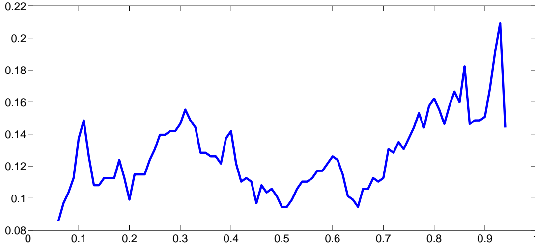
Figure 2.10: Unconditional QTE
