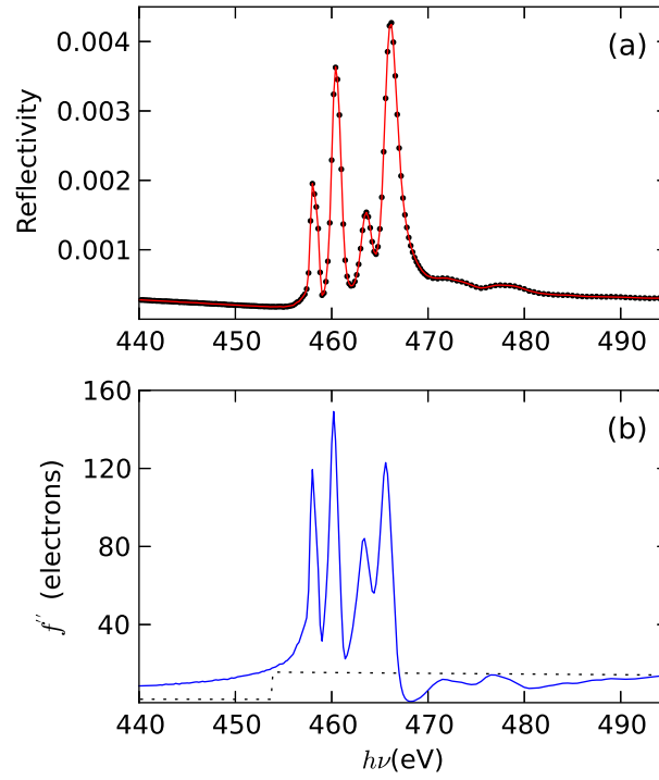
FIG. 2. (Color Online) Results of refinement of model #1. Reflectivity, (a), across the Ti L_{2,3} edge measured at \theta = 14^\circ (black circles) and calculated from the refined model (red line). The resulting spectrum for the imaginary part of the atomic scattering factor, f'' , (solid line) is shown in (b), along with the step function from the tabulated data (dotted line) for that edge for comparison. Only the data shown was considered for the refinement of this model.
