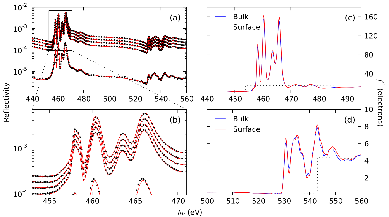
FIG. 5. (Color Online) Results of refinement of model #3b. Reflectivity, (a), across the Ti L_{2,3} and O K edges measured at \theta = 14^\circ, 15^\circ, 16^\circ, 17^\circ, and 30^\circ (black circles) and calculated from the refined model (red line) are shown top to bottom. The Ti L_{2,3} edge is shown in finer detail in (b). All data shown were considered in the refinement of this model. The resulting spectra for the imaginary part of the atomic scattering factors, f'' , are shown in (b) for Ti and (c) for O, along with the step functions from the tabulated data for that edge for comparison.
