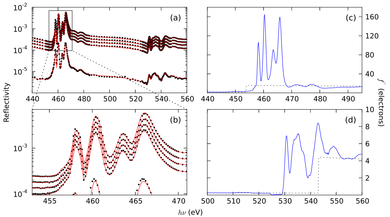
FIG. 4. (Color Online) Results of refinement of model #3a. Reflectivity, (a), across the Ti L_{2,3} and O K edges measured at \theta = 14^\circ, 15^\circ, 16^\circ, 17^\circ, and 30^\circ (black circles) and calculated from the refined model (red line) are shown top to bottom. The Ti L_{2,3} edge is shown in finer detail in (b). All data shown were considered in the refinement of this model. The resulting spectra for the imaginary part of the atomic scattering factors, f'' , are shown in (b) for Ti and (c) for O, along with the step functions from the tabulated data for that edge for comparison.
