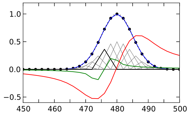
FIG. 1. (Color Online) A gaussian function (dashed line), sampled at discrete points (circles), and approximated by a sum of basis triangle functions (grey), leading to a linear approximation to the original function (blue). The KK transform of a single triangle function (green) as well as the sum of all such functions representing the KK transform of the full gaussian function (red) are also shown.
