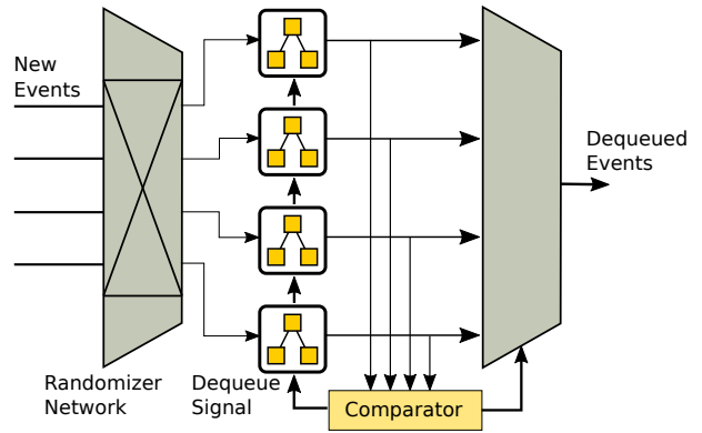
Figure 4: Multiple event issue priority queue
