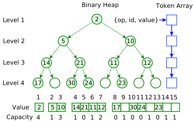
Figure 3: The P-heap data structure[23]
