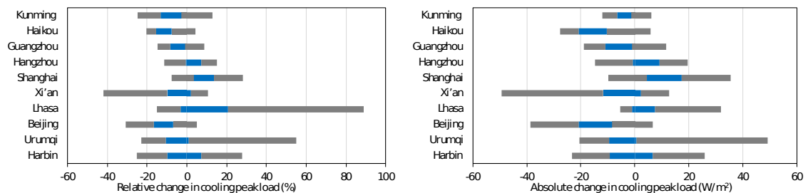
Fig. 12. Relative and absolute change in the cooling peak load for the 10 cities
