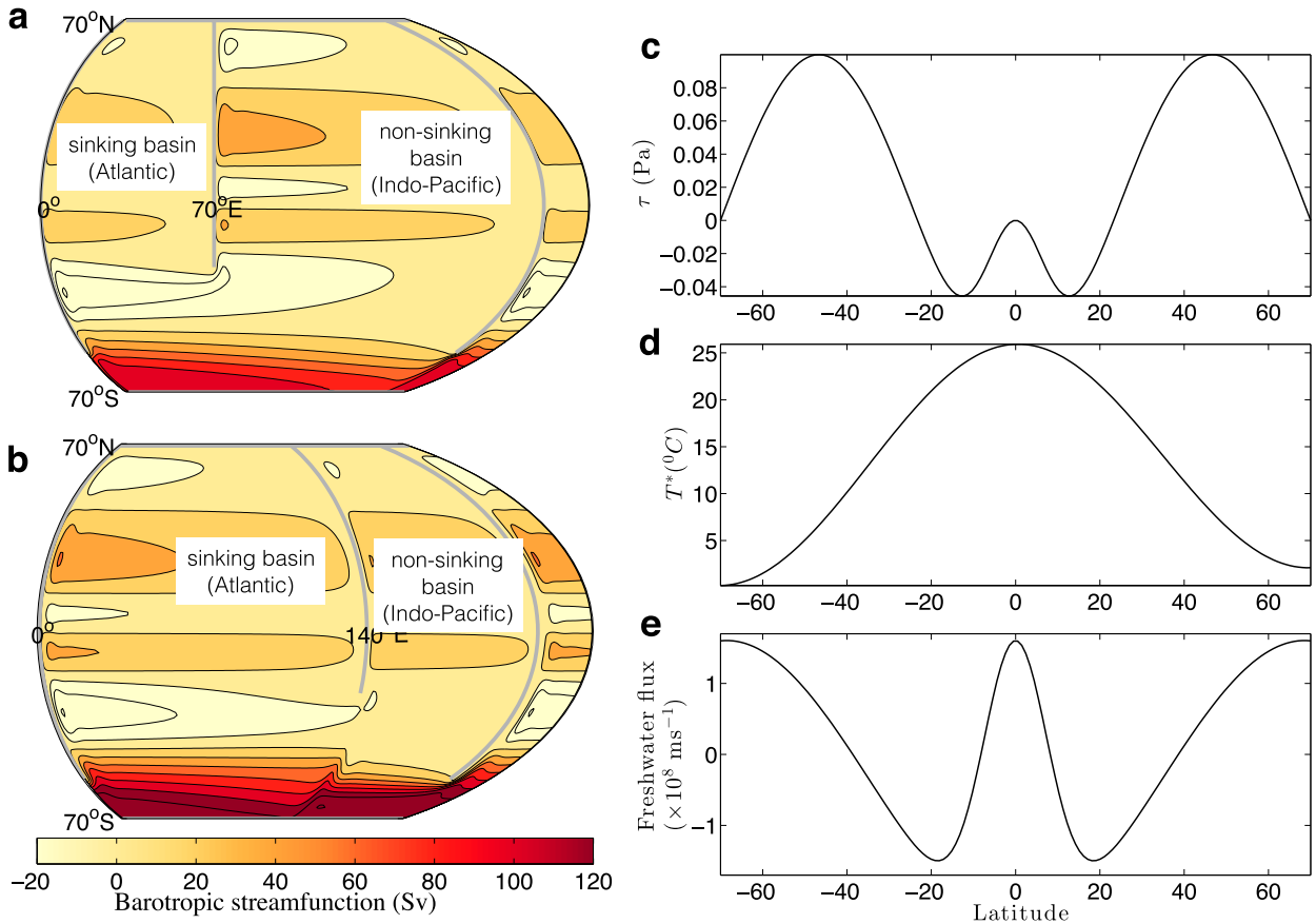
FIG. 1. The barotropic streamfunction in the geometry of (a) the standard configuration and (b) the exchanged configuration. The gray lines indicate solid boundaries. The domain is 140° in latitude, 210° periodic in longitude, and 4000 m deep. The westernmost 20° of the domain is repeated on the right side of the panels. In both cases, deep water is formed in the basin to the west of the short continent. Also shown are (c) surface wind stress (Pa), (d) the profile of temperature used for temperature relaxation (°C), and (e) surface freshwater flux forcing ( \times 10^8 \text{ m s}^{-1} ).
