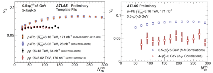
Figure 7. Left: Charged particle v_2\{2\} from pp and p+Pb collisions at various collision energies as a function of number of reconstructed charged particles. Right: v_2\{2\} for heavy flavor muons compared with charged hadrons in p+Pb collisions. All results obtained using the template fit method.
