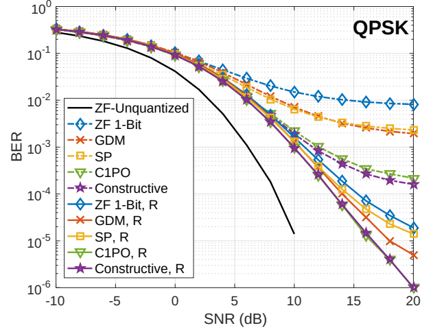
Fig. 3: BER v.s. transmit SNR, N_t = 8 , K = 2 , QPSK
