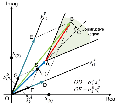
Fig. 2: 8PSK as an example for the signal decomposition
