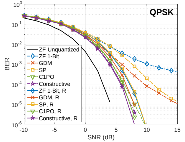
Fig. 4: BER v.s. transmit SNR, N_t = 128 , K = 16 , QPSK
