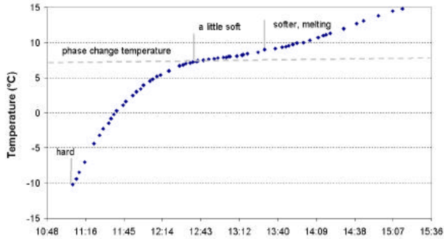
Figure A4.1.3 Phase change material surface temperature during phase change process
