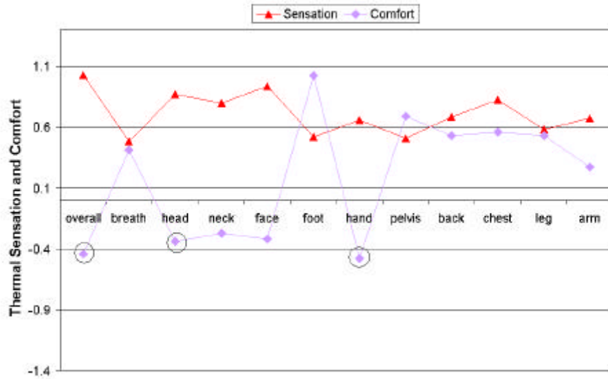
Figure 6.54 Validation of overall comfort model for UC Berkeley chamber experiment data in slightly warm environment (overall sensation near 1, 3 tests)
