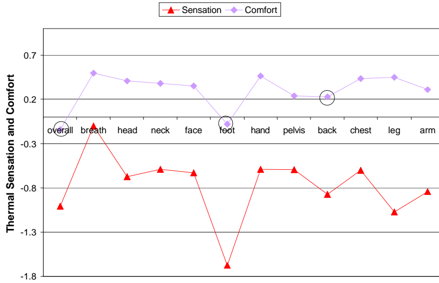
Figure 6.53 Validation of overall comfort model for UC Berkeley chamber experiment data in slightly cool environment (overall sensation near -1, 6 tests)
