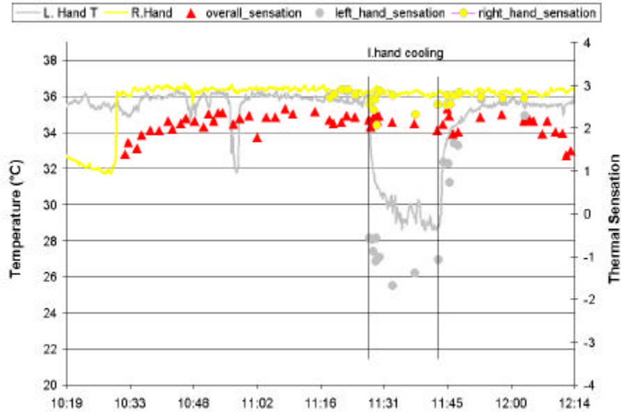
Figure 5.46 Left and right hand sensations during left-hand cooling (23108)
