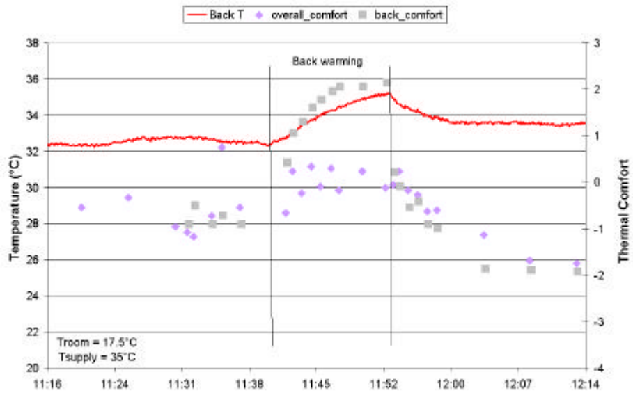
Figure 5.22-4 Back and overall thermal comfort during back heating (23089)
