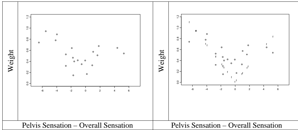
Figure 6.39 Linear relationships to calculate the weights based on the difference between local sensation and the overall sensation
