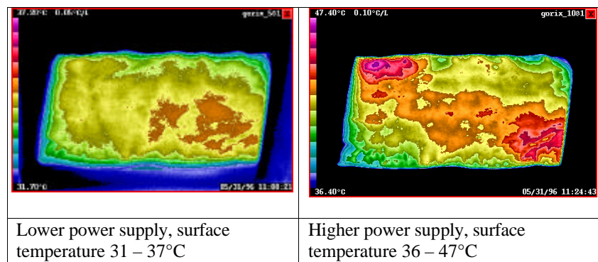
Figure A4.1.2 Uneven surface temperature of an electrical fabric
