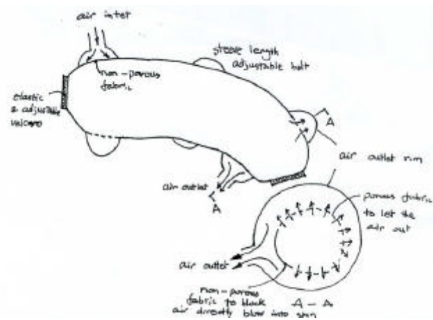
Figure 4.5 Design details of the air sleeve
