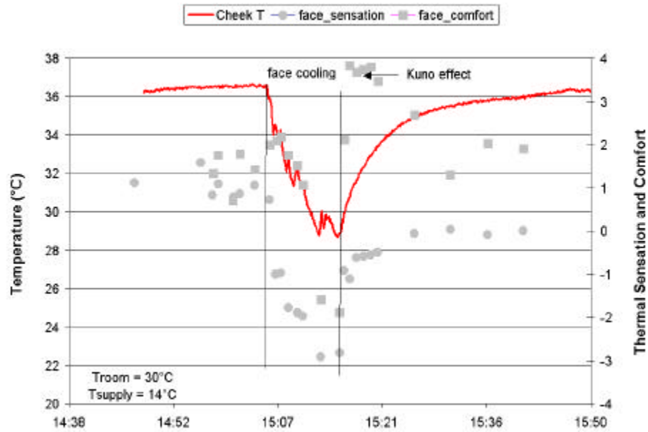
Figure 5.36 Kuno effect during strong face cooling removal (13037)
