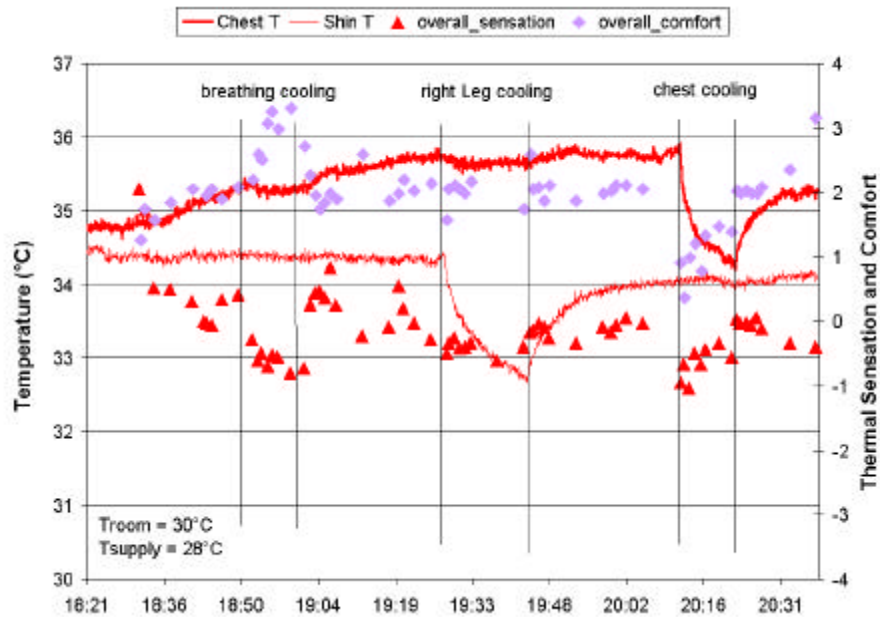
Figure 5.31-3 Overall thermal sensation and comfort for three local cooling applications in one test (09022)
