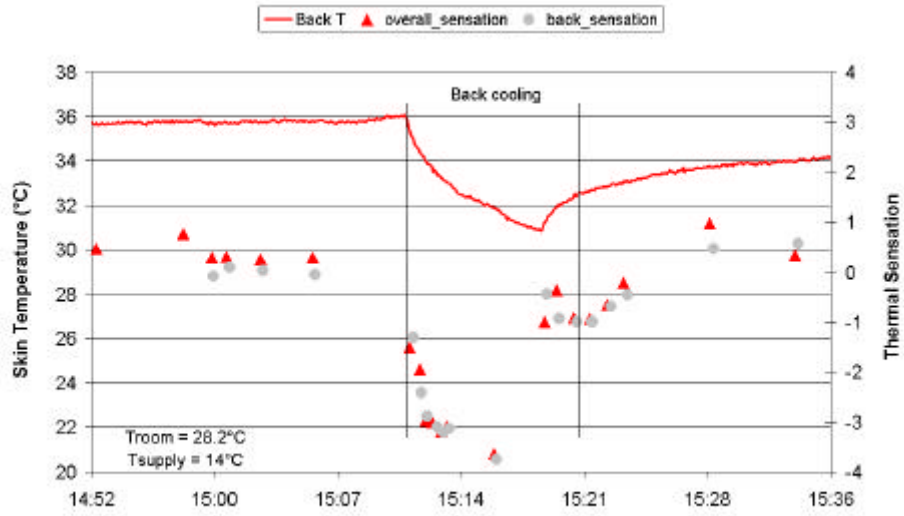
Figure 5.20-1 Back and overall thermal sensation during back cooling (03001)
