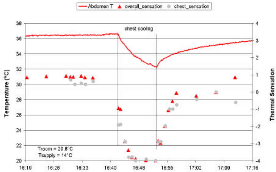
Figure 5.20-2 Chest and overall thermal sensation during chest cooling (13037)
