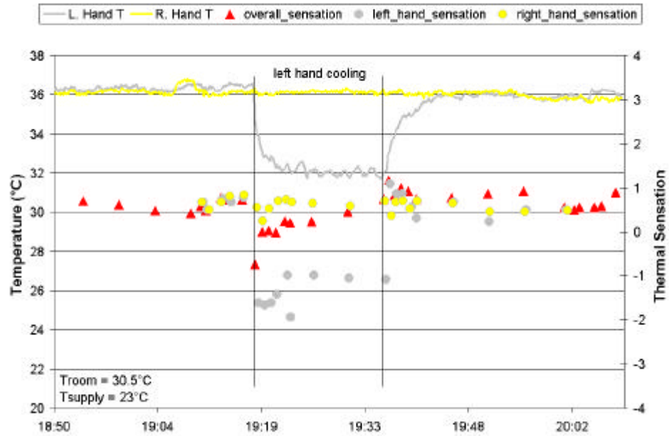
Figure 5.47-1 Left and right hand sensations during left-hand cooling (18066)
