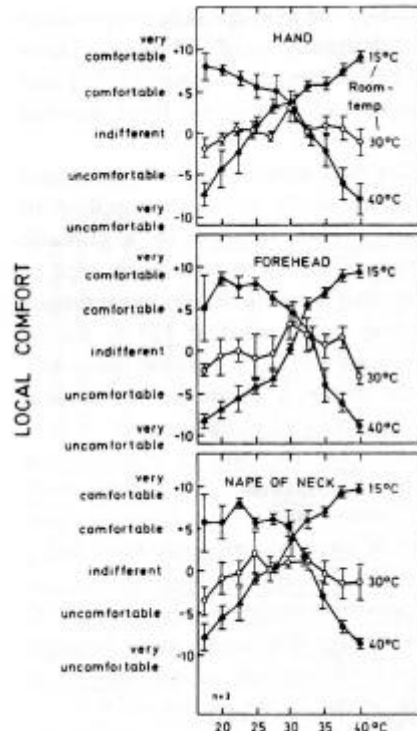
Figure 6.24 Local comfort vs. local skin temperature and whole body thermal states (Hildebrandt, Engel et al. 1981), data from Attia and Engel (Attia and Engel 1981)
