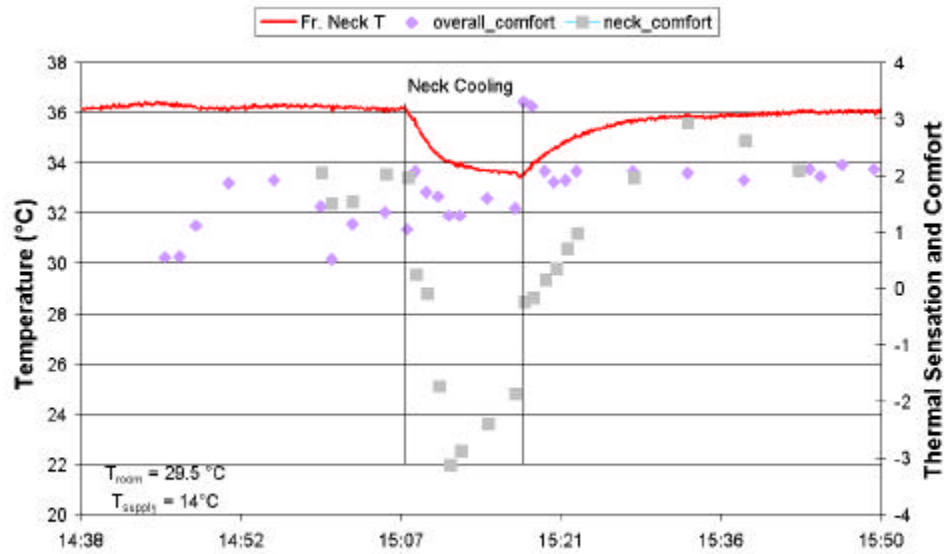
Figure 5.27-6 Neck and overall thermal comfort during strong neck cooling (13030)
