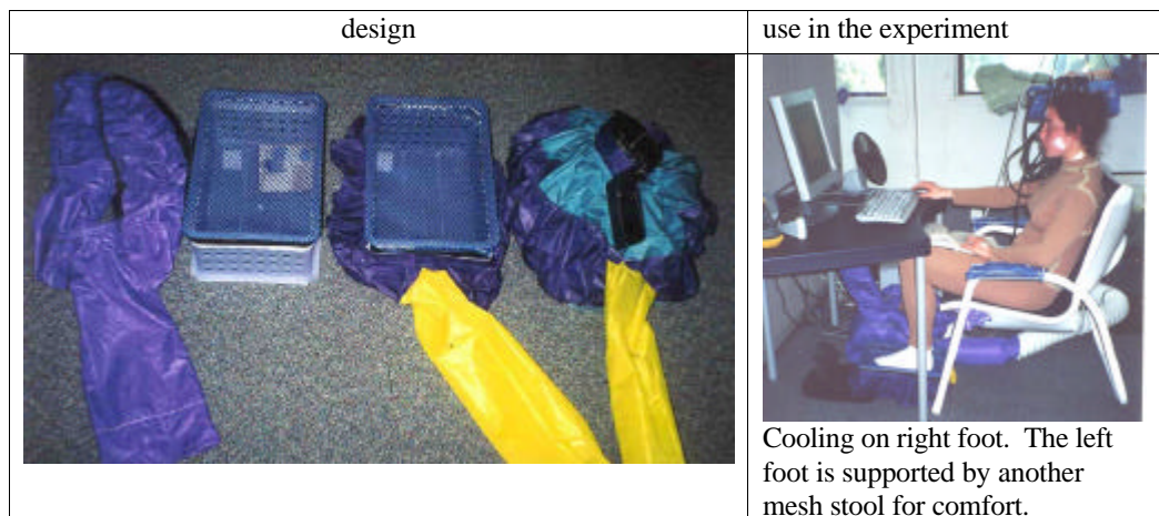
Figure 4.17 Foot air sleeve
