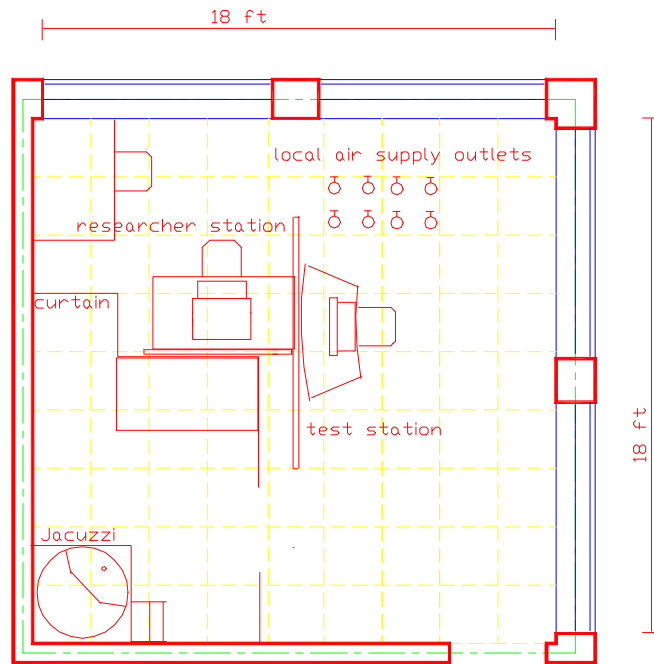
Figure 4.1 The controlled environmental chamber setup
