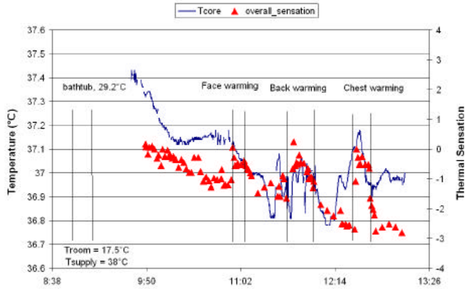
Figure 5.33-1 Core temperature and overall sensation during local warming (23089)
