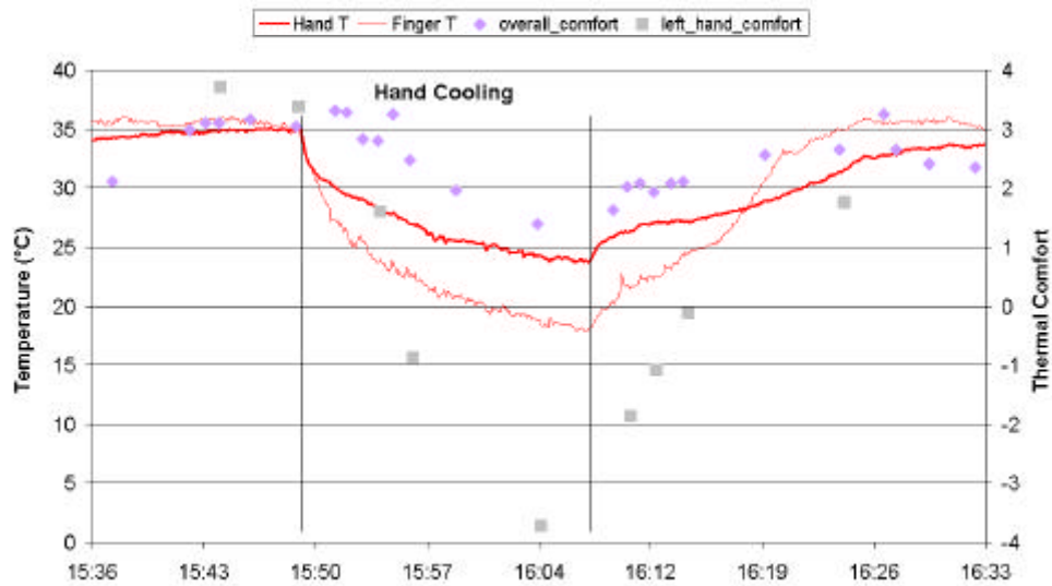
Figure 5.24-6 Hand and overall thermal comfort during hand cooling (13016)
