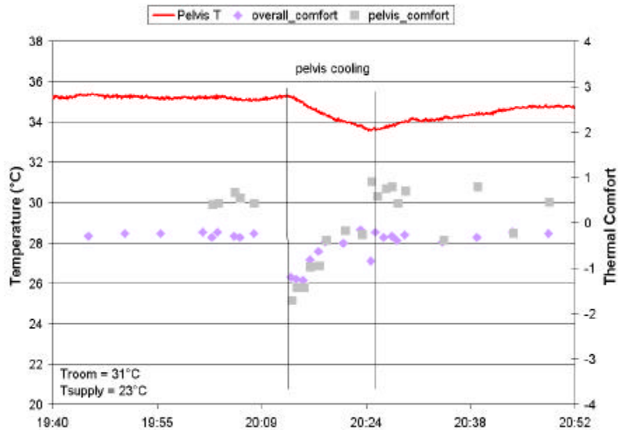
Figure 5.20-7 Pelvis and overall thermal comfort during pelvis cooling (18066)
