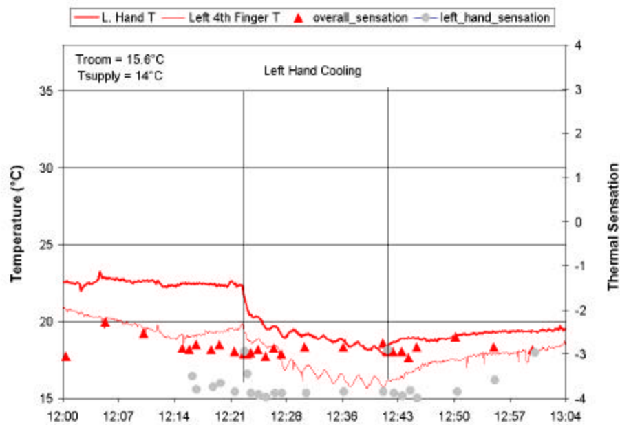
Figure 5.25-3 Hand and overall thermal sensation during hand cooling in cold environment (21083)
