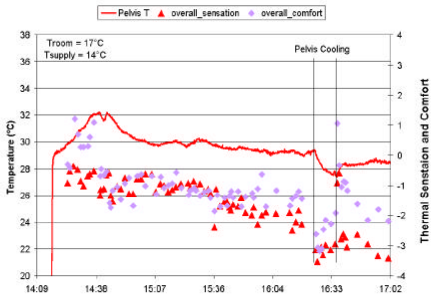
Figure 5.21 Pelvis and overall thermal sensation during pelvis cooling in a cold environment (17084)
