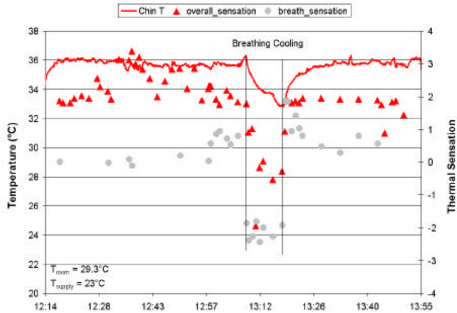
Figure 5.31-1 Breathing and overall thermal sensation during breath intake air cooling (21073)
