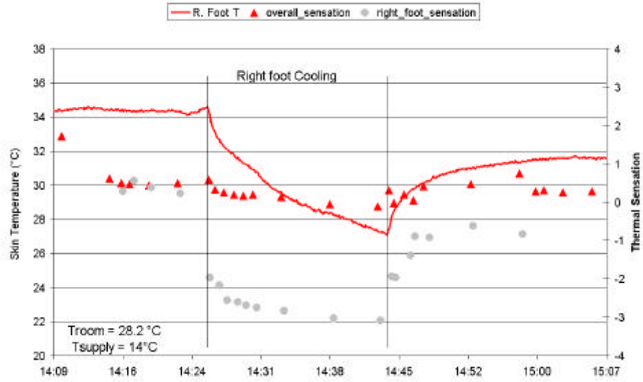
Figure 5.24-1 Foot and overall thermal sensation during foot cooling (03001)
