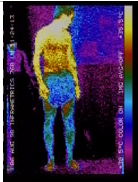
Figure 5.13 Skin temperature distribution in warm environment
