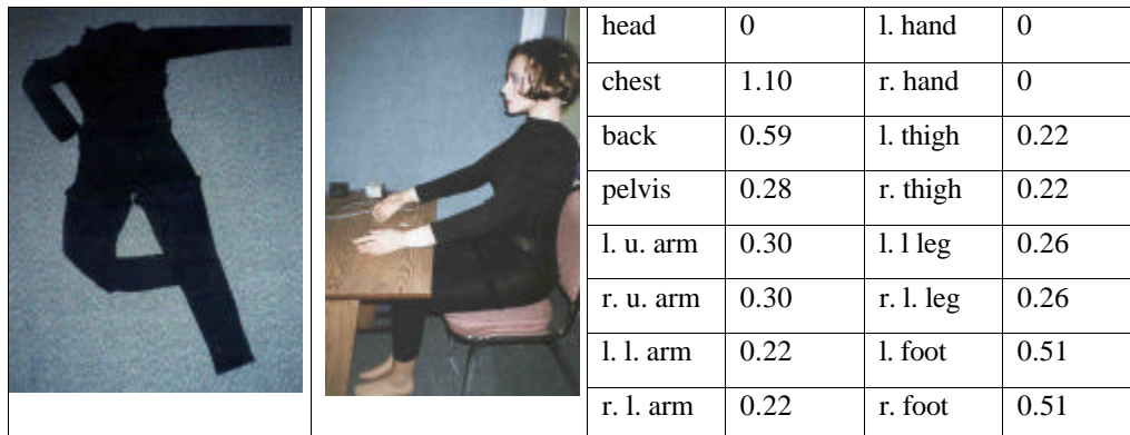
Figure 4.6 The thermal manikin measuring the clothing insulation value of the leotard, with insulation values (clo) listed.
