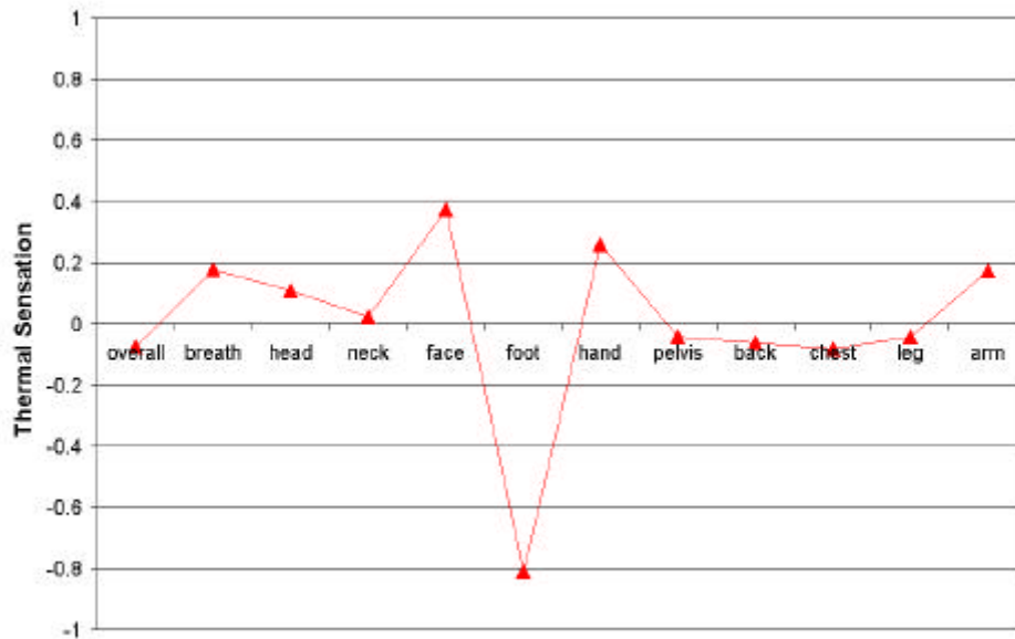
Figure 5.4 Thermal sensation under neutral conditions ( 8 tests)
