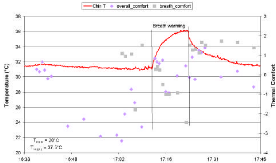
Figure 5.30 Breathing and overall thermal comfort during breath intake air warming (27091)
