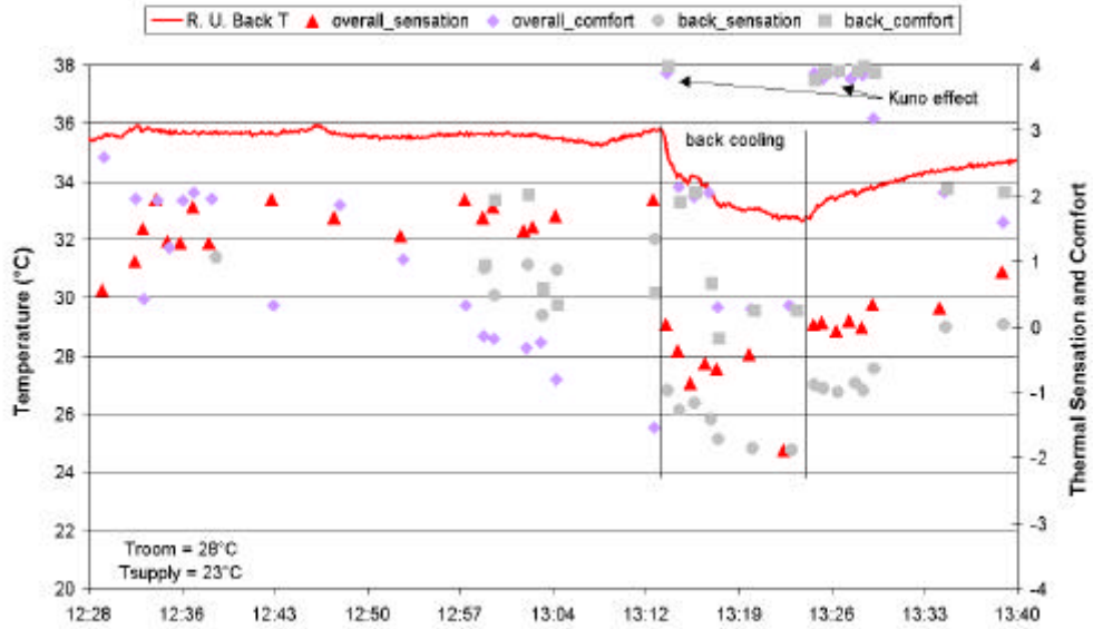
Figure 5.38 Kuno effect during mild back cooling removal (10063)
