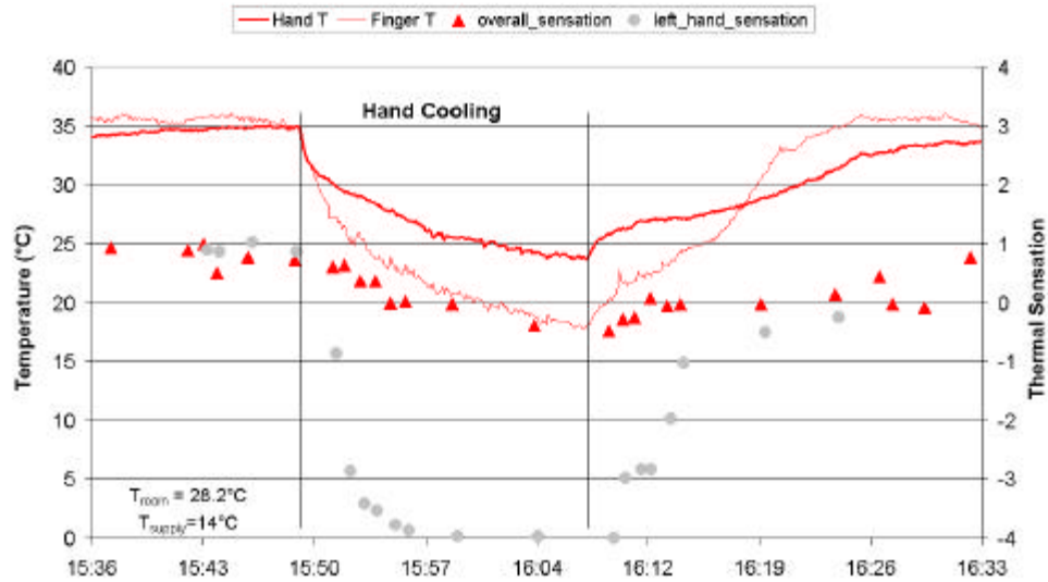
Figure 5.24-5 Hand and overall thermal sensation during hand cooling (13016)
