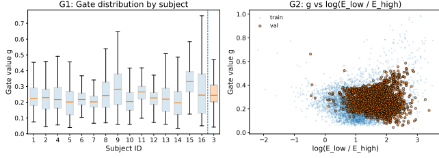
Figure 3: BandGate on KUL (LOSO): (G1) subject-wise gate distribution; (G2) gate vs. log band-energy ratio.
