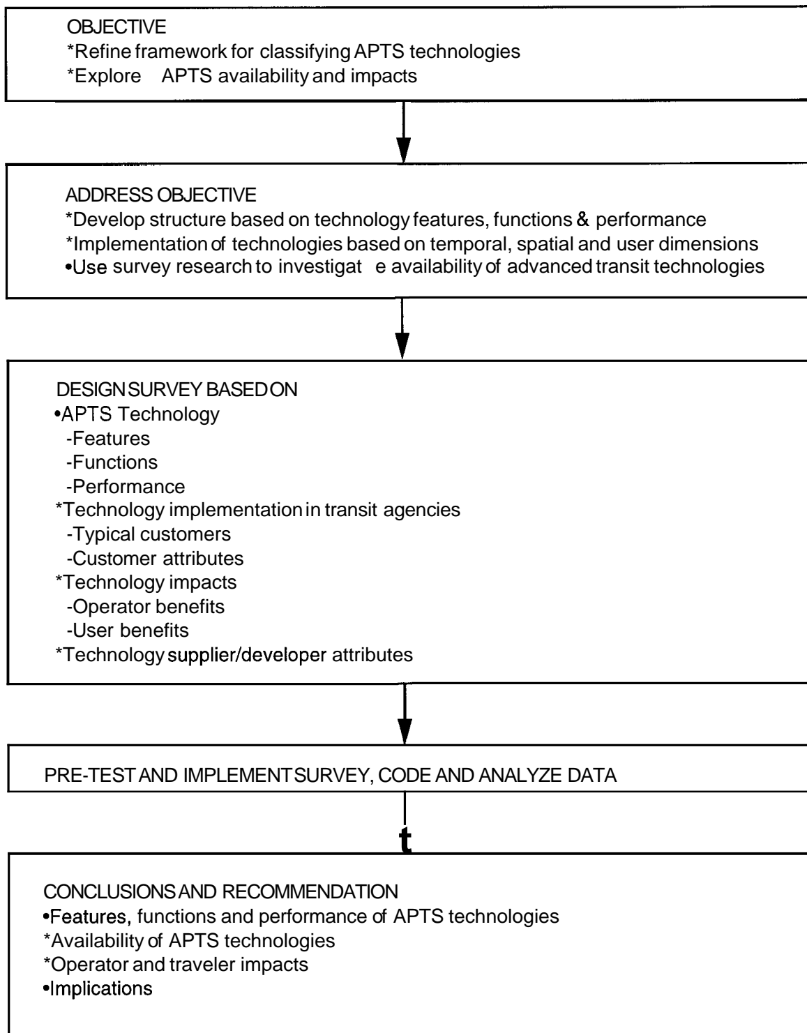
Figure 3. Study methodology.
