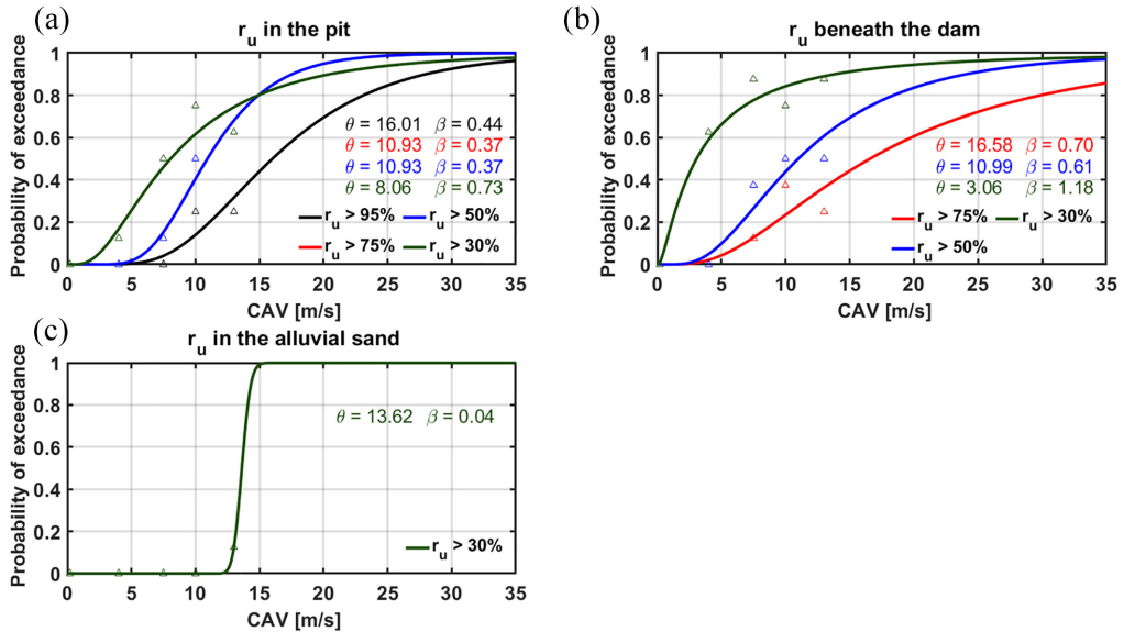
Figure 8. Fragility functions for the excess pore water pressure ratio r_u for the Angitola dam using CAV as Intensity Measure: (a) pit; (b) beneath the dam; (c) alluvial sand.
