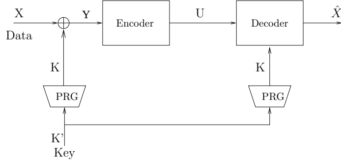
Fig. 3. Secure compression scheme: The data X is first encrypted with a stream cipher and then compressed. At the receiver, decoding and decryption are performed in a joint step. The eavesdropper sees U , but (as we show) cannot learn anything useful about X .
