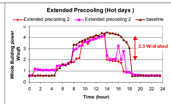
Figure 8. Extended Pre-Cooling Tests on Hot days
