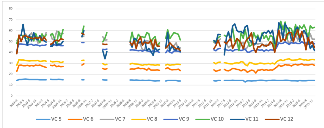
Figure 5. Monthly GVW average Feb-03 to Dec-15, WIM station 12
