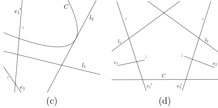
Figure 1.2: Blowing up in Example 1.1.13.
