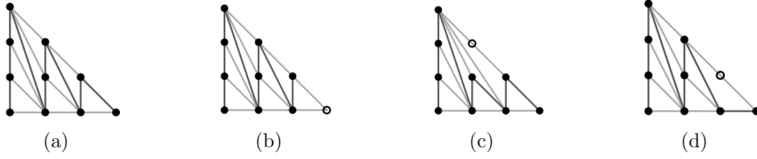
Figure 5.9: The triangulation dual to a smooth cubic floor and the three possible subdivisions dual to a tropical cubic curve with one node germ.
