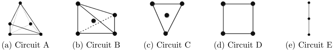
Figure 5.4: Circuits in the dual subdivision inducing nodes in the surface.
