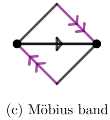
Figure 2.13: We see (S^1)_2 is a Möbius strip through cutting and rearranging the pieces.
