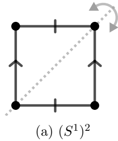
Figure 2.13: We see (S^1)_2 is a Möbius strip through cutting and rearranging the pieces.
