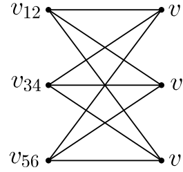
Figure 4.13: Tropicalization of the curve in Example 4.5.18.
