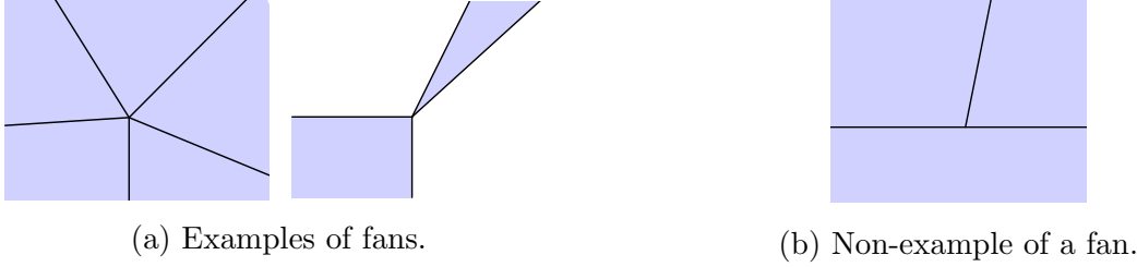
Figure 1.5: Examples and non-examples of polyhedral fans.
