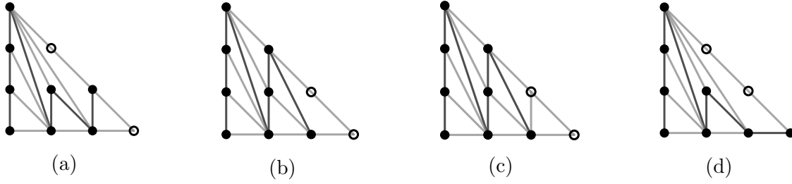
Figure 5.15: Cubics with two node germs.
