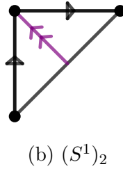
Figure 2.13: We see (S^1)_2 is a Möbius strip through cutting and rearranging the pieces.
