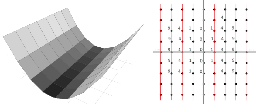
Figure 2.3: The weight function induced by the quadratic form in Example 2.1.12 on the left, and the corresponding Delaunay subdivision on the right.
