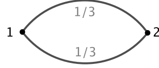
Figure 4.16: Tropical genus 4 Shimura-Teichmüller curve.
