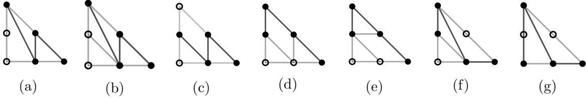
Figure 5.14: Dual subdivisions of conics with two node germs.
