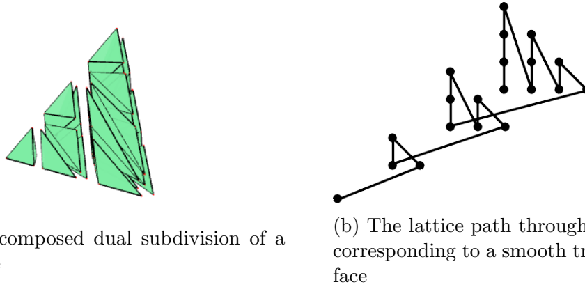
Figure 5.3: Subdivision and lattice path to a smooth tropical cubic surface through points in Mikhalkin position.
