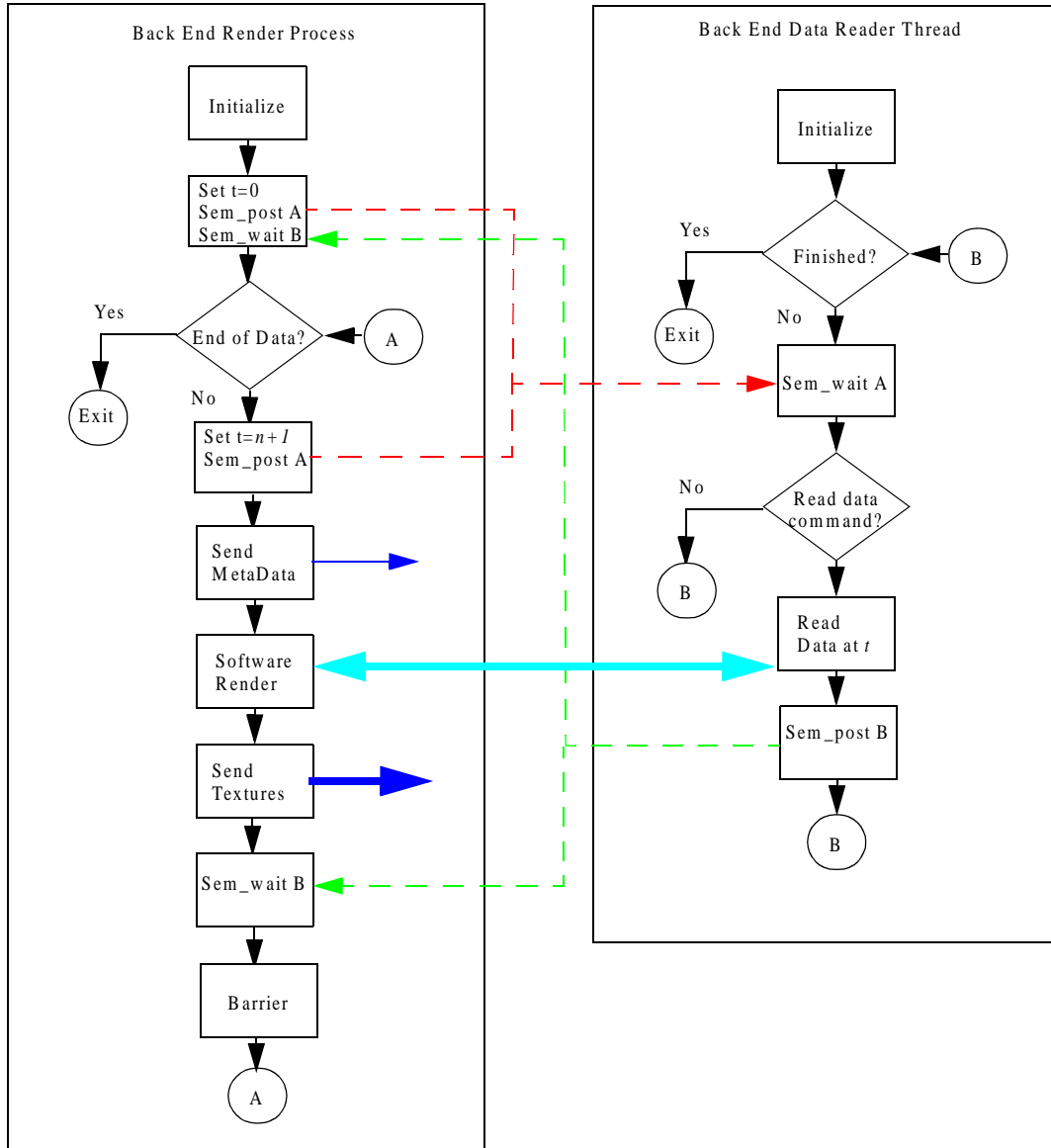
FIGURE 19. Architecture of Overlapped Visapult Back End
