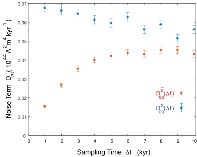
Fig. 5. Estimates for the noise term, D_{eq}(\Delta t) , computed from exact x(t) and filtered \bar{x}(t) time series. Temporal averaging substantially reduces the noise term when \Delta t is less than the averaging time T = 3 kyr. Estimates for D_{eq}^x(\Delta t) approach a constant value once \Delta t > 2T .
