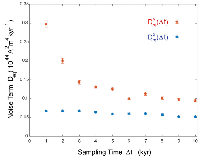
Fig. 2. Estimates for the noise term, D_{eq}(\Delta t) , computed from exact x(t) and noisy y(t) time series. Addition of random error to y(t) causes D_{eq}^y to depart from the known value D_{eq} = 0.069 \times 10^{44} \text{ A}^2 \text{ m}^4 \text{ kyr}^{-1} . Calculations using x(t) reproduce the known value to within the uncertainties at \Delta t = 1 \text{ kyr} . Discrepancies in D_{eq}^x(\Delta t) increase slowly with \Delta t due to unmodelled contributions from higher-order powers in \Delta t .
