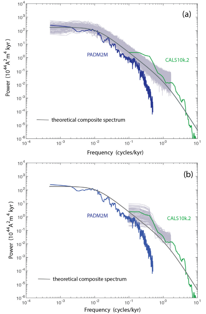
Fig. 8. (A) Power spectra from 100 realizations of the stochastic model (light gray) compared with the power spectra computed from PADM2M (blue) and CALS10k.2 (green). A theoretical spectrum (dark gray) is based on the parameters of the revised stochastic model and the influences of correlated noise with a correlation time of T = 120 years. The ensemble of realizations is compatible with PADM2M at low frequencies. (B) Power spectra of 100 shorter (10-kyr) realizations of the stochastic model agree well with the power spectrum for CALS10k.2.
