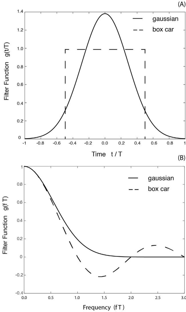
Fig. 3. (A) Two commonly used filters are the Gaussian, g(t) = (6/\pi T^2)^{1/2} \exp(-6t^2/T^2) , and the box car, g(t) = 1/T for |t| < T/2 , where T is the averaging time. (B) Fourier transforms are given by g(f) = \exp(-4\pi^2 f^2 T^2/24) and g(f) = \sin(\pi f T)/\pi f T , respectively.
