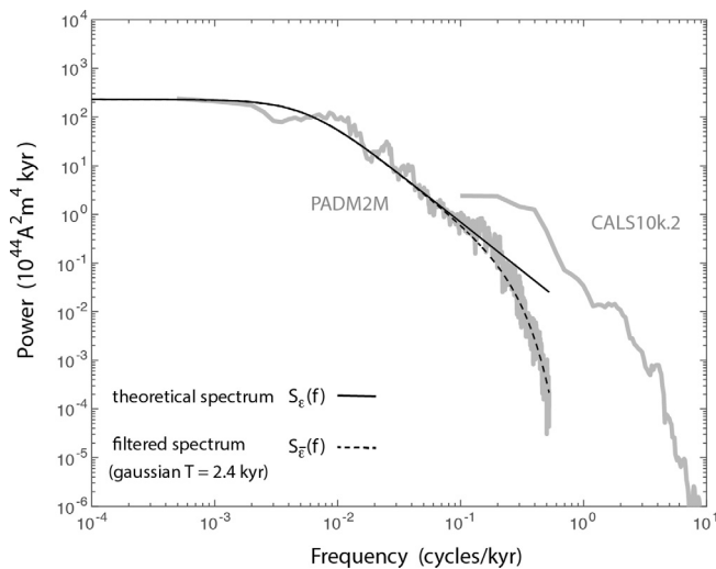
Fig. 6. Power spectra computed from PADM2M and CALS10k.2 using a multi-taper method. Theoretical spectra S_e(f) and S_e(f) are based on the stochastic model derived from PADM2M and a filtered version of the stochastic model. We apply a Gaussian filter with an averaging time of T = 2.4 kyr to account for the abrupt decrease in power of PADM2M at high frequency.
