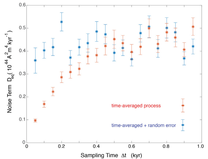
Fig. A.1. Recovery of noise term D_{eq} from a 10-kyr realization of the preferred stochastic model. A box-car filter is applied to the realization with and without the addition of random error. Sampling the process at \Delta t = 2T = 300 years gives a reasonable estimate for D_{eq} , even when a realistic level of random error is added to the process.
