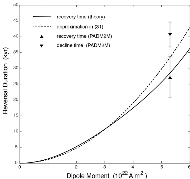
Fig. 10. Mean recovery time for the dipole moment following a reversal. A numerical solution of the Fokker-Planck equation (theory) is compared with the approximation in (31), where the drift term is assumed to vanish. Discrete estimates from PADM2M are shown for the recovery and decline times. The recovery time agrees well with the theoretical estimate for recovery, whereas the decline time exceeds the recovery time due to contributions from the drift term.
