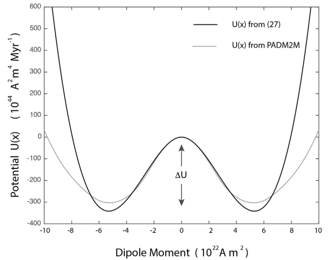
Fig. 9. Potential U(x) computed from (27) compared with a potential recovered from PADM2M. Both potentials have comparable barriers, \Delta U , but different amplitudes at large |x| . The width of the potential well is defined by the second derivative U''(x) = -\gamma at x = \pm \langle x \rangle . We use \gamma = 0.075 \text{ kyr}^{-1} for the potential in (27).
