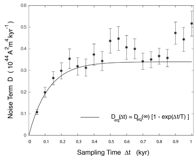
Fig. 7. Estimates for the noise term, D_{eq} , recovered from CALS10k.2 as a function of sampling time \Delta t . A simple parametric fit to D_{eq}(\Delta t) in (23) gives D_{eq}(\infty) = 0.34 \times 10^{44} \text{ A}^2 \text{ m}^4 \text{ kyr}^{-1} . The effective correlation time of the noise source is T = 120 years.
