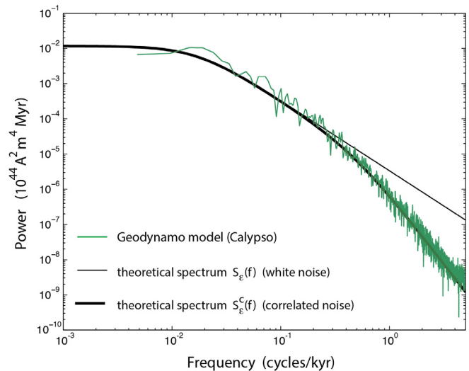
Fig. 1. A power spectrum of dipole fluctuations from a numerical geodynamo simulation (Matsui et al., 2014), compared to predictions from two stochastic models. One stochastic model assumes a white noise source and the other assumes correlated noise. Both models are capable of predicting the low-frequency fluctuations even though the drift and diffusion terms are constructed from short-period information.
