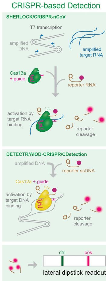
FIGURE 8. Molecular overview of CRISPR detection of amplified products. Binding to specific target sequences in amplified RNA or DNA activates Cas nucleases, which cleave reporter molecules. Reporter cleavage can then be assayed using a lateral dipstick.
