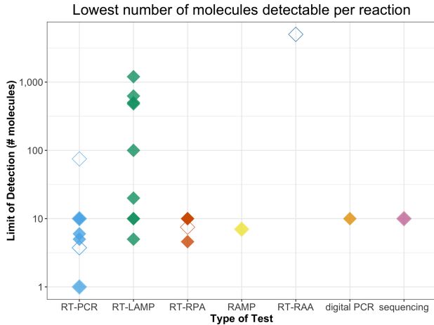
FIGURE 6. The limit of detection for published tests equivalent to the fewest number of molecules accurately assayed in a single reaction. For some spike-in controls, authors used viral DNA, plasmid DNA, or a pseudovirus instead of viral RNA (shown as open diamonds), which may have a different amplification efficiency than SARS-CoV-2 RNA and thus alter their calculated limit of detection. Raw data available in Supplemental Table S1.
