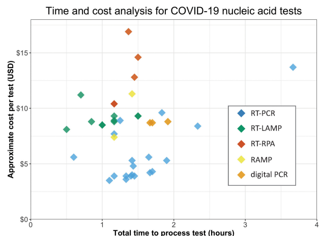
FIGURE 3. An analysis of the total workflow time and calculated cost (in U.S. dollars) of published COVID-19 nucleic acid tests. Calculated costs are estimated from available online pricing for consumables and do not include labor or equipment. Protocols which required key reagents to be synthesized or created in a laboratory are not included but are likely to be even cheaper than commercially priced reagents. All raw data available in Supplemental Tables S1, S2.
