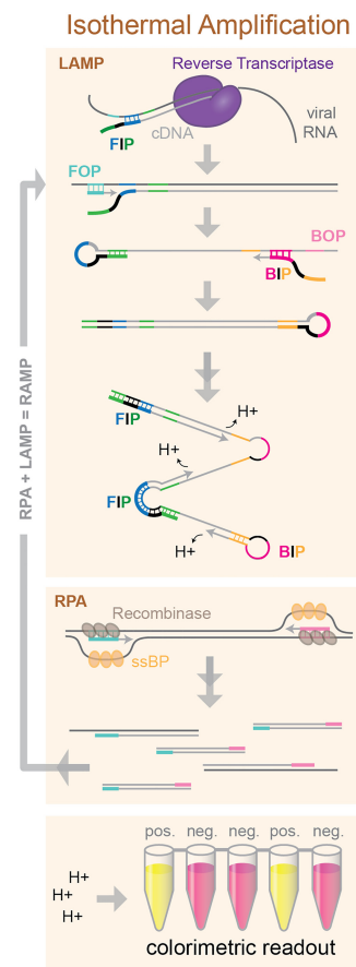
FIGURE 7. Molecular overview of isothermal amplification techniques. LAMP uses specially designed nested primers with complementary regions that form hairpins to permit priming of subsequent rounds of amplification. RPA uses recombinase-catalyzed strand invasion to prime amplification. Colorimetric pH indicators can be used to detect hydrogen ion release during dNTP incorporation.
