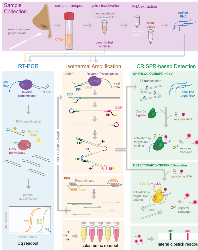
FIGURE 1. An overview of COVID-19 nucleic acid testing. Samples collected via nasopharyngeal swab are lysed and inactivated, and an amplification reaction is performed using either a crude swab sample or purified RNA. Amplification of specific viral sequences by RT-PCR, LAMP, or RPA is detected using fluorescent or colorimetric dyes, sequence-specific CRISPR-Cas nuclease cleavage of a reporter, or separation of reaction products on a lateral flow dipstick.
