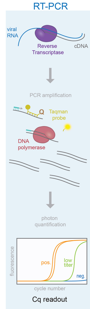
FIGURE 5. Molecular overview of the RT-PCR reaction. Taqman probes are used to visualize increased fluorescence during each cycle of amplification. Amplification is quantified by C_q readout and a threshold is set for positive detection of the target amplicon.
