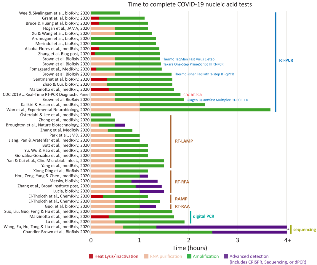
FIGURE 4. Examination of the total workflow for published COVID-19 testing methods. Each step of the workflow is shown with colored bars. Four example commercial RT-PCR kits are included for reference (blue) and were directly compared within a single publication. The CDC RT-PCR test is shown in red. (*) Sequencing typically takes 4–12 h but can vary significantly depending on library preparation and the platform used, and was not specifically stated in the cited protocols. Raw data available in Supplemental Table S1.
