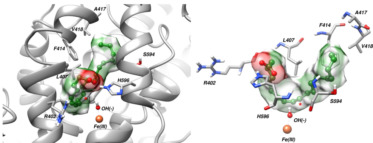
Figure 1. Two representations of the predicted binding mode of the AA C-10 carbanion intermediate in the hALOX12 wild-type enzyme active site. The negatively charged carbanion C10 is identified with a star (*). H596 is predicted to form a hydrogen bond to the carboxylate group of the fatty acid. The AA carbanion intermediate is shown in a ball-and-stick and surface representations. The hydroxide ion is shown in a ball-and-stick representation while the key residues that are mutated in this study are shown in a stick representation. Carbon atoms of AA and the protein are shown in grey and green, respectively. Iron is depicted as an orange sphere. Nitrogen, oxygen atom
