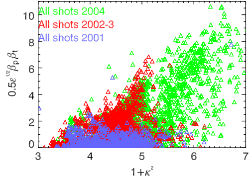
Figure 6. The parameter 0.5\sqrt{\epsilon}\beta_p \times \beta_t plotted versus 1 + \kappa^2 . Each point represents the pulse average of one NSTX plasma discharge, with every discharge in the NSTX database plotted.
