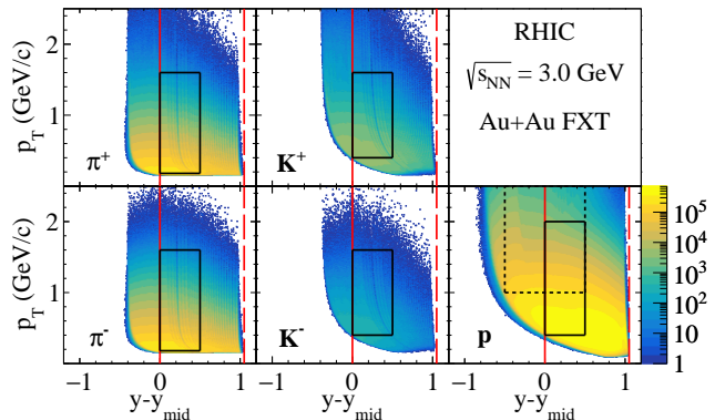
FIG. 2. p_T vs. y_{c.m.} density plots for \pi^\pm , K^\pm , and p measured by the STAR in Au+Au collisions at \sqrt{s_{NN}} = 3.0 GeV. The red dashed line represents the target rapidity and the solid red line represents midrapidity. The solid and dashed black boxes mark acceptance regions used for flow calculations in various cases explained in the text.
