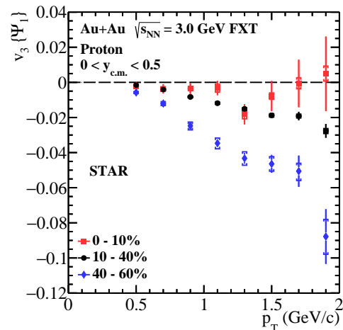
FIG. 8. v_3\{\Psi_1\} vs. p_T for protons in three large centrality bins. v_3\{\Psi_1\} becomes increasingly negative as p_T and centrality increase. Statistical uncertainties are shown as lines while systematic uncertainties are denoted by open square brackets.
