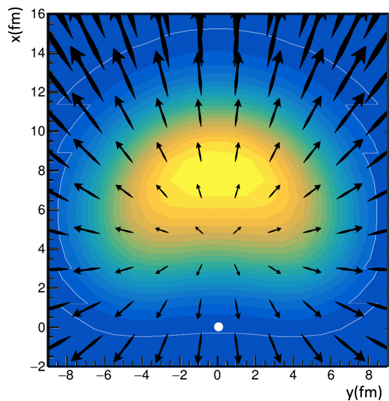
FIG. 13. Illustration of the x vs. y position of protons from JAM at t = 50 fm/c for particles with rapidity 0.6 < y < 0.85 and 0 < p_T < 2 GeV/c (avoiding spectators) illustrating the half-moon, “triangular” shape. Note that the high density region is centered at x \approx 7 fm. The arrows depict the vector field obtained by dividing the collision region into cells. The average momentum in each cell is superimposed on the original plot. The length of each arrow represents the magnitude of the average momentum in each cell. The white dot indicates the x = 0 , y = 0 position.
