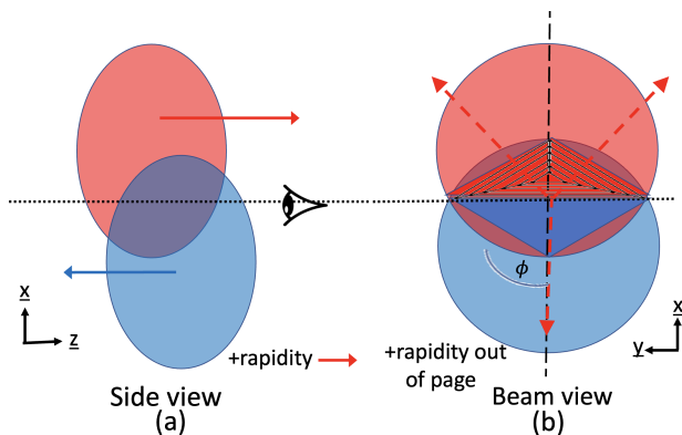
FIG. 12. Illustration of the triangular geometry of participants as discussed in the text.
