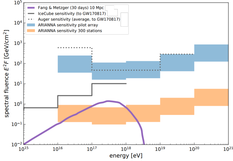
Figure 1.3: Expected spectral fluence of neutrinos from gravitational wave event GW170817 (purple line)[7], as well as sensitivities of the IceCube neutrino observatory and Pierre Auger observatory [8]. The effective volume from an array of 300 ARIANNA style radio surface stations is expected to be sufficiently high to have expected an observation for this event. From [9].
