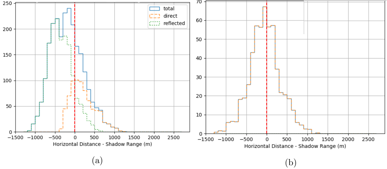
Figure 4.8: Distance distribution for simulated neutrino events for Moore’s Bay (a), and South Pole (b) ice for an effective horizontal attenuation length \lambda_h = 400 m. Positive values represent events which originate in the “shadow zone” (see Section 3.2.5). The additional area under the curve to the right of the vertical red line represents the effective volume gained by these classically forbidden triggers.
