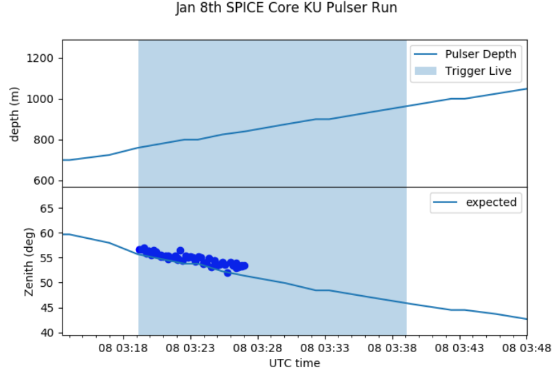
Figure 2.22: KU SPICEcore pulser location vs time, along with expected and reconstructed zenith angle.
