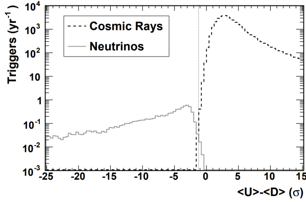
Figure 5.13: Difference in average signal amplitude in upward and downward facing antennas for neutrinos and cosmic rays, from [24]. A cut of < -1.2\sigma maintains 99.7% of the neutrino signal, while reducing the cosmic ray background rate to 0.1 events over a three year run of 1296 ARIANNA stations.
