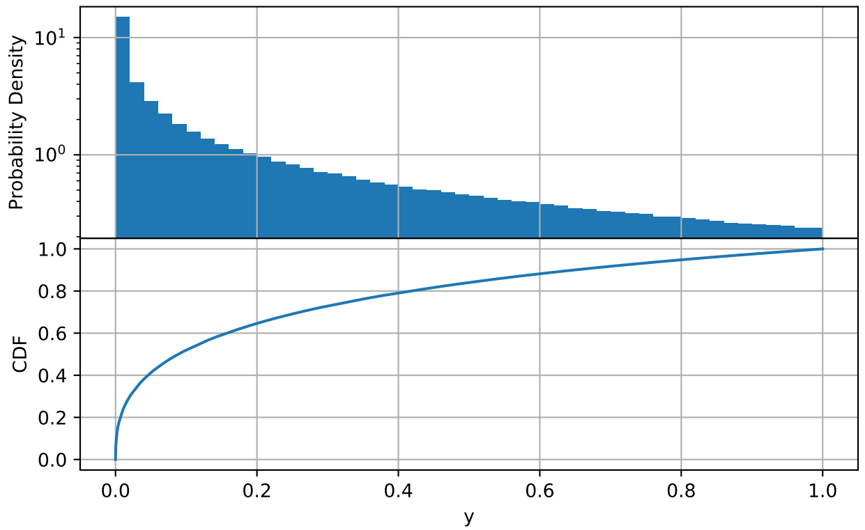
Figure 3.1: Probability distribution (top) and cumulative distribution function (bottom) for the inelasticity ( y ). Half of neutrino induced showers will have E_{sh} = yE_\nu < 0.1E_\nu in the hadronic shower.
