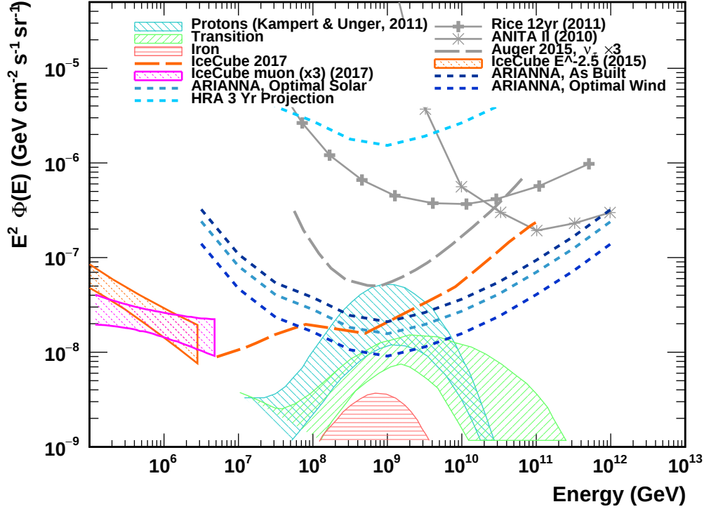
Figure 1.10: Current status of measured fluxes and 90% confidence upper limits on the flux of astrophysical and cosmogenic neutrinos. Experiments are continuing to probe models for the GZK flux, but predictions at 10^{18} eV span over an order of magnitude. IceCube spectra from [14, 15]. Icecube limit from [16]. RICE, Auger, and ANITA limits from [17, 18, 19]. GZK flux models from [12]. For details of the calculation see section 5.4.1.
