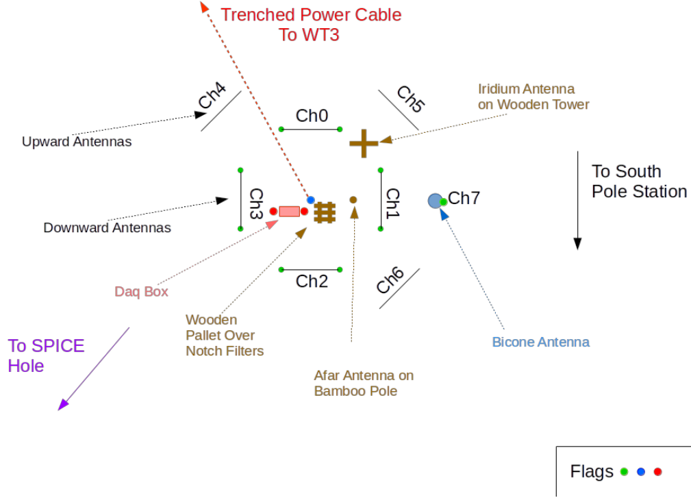
Figure 2.31: Digram of the ARIANNA South Pole pilot station, showing the antenna positions and orientation relative to South Pole landmarks.
