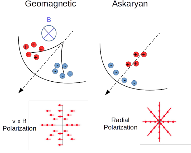
Figure 1.4: Diagram of the two main methods for coherent radio emission in particle showers. The geomagnetic mechanism (left) relies on the time dependent transverse currents induced by the Earth’s magnetic field. Geomagnetic emission has a characteristic polarization in the \vec{v} \times \vec{B} direction. Askaryan emission arises due to charge separation along the shower axis, leading to a radial polarization profile.
