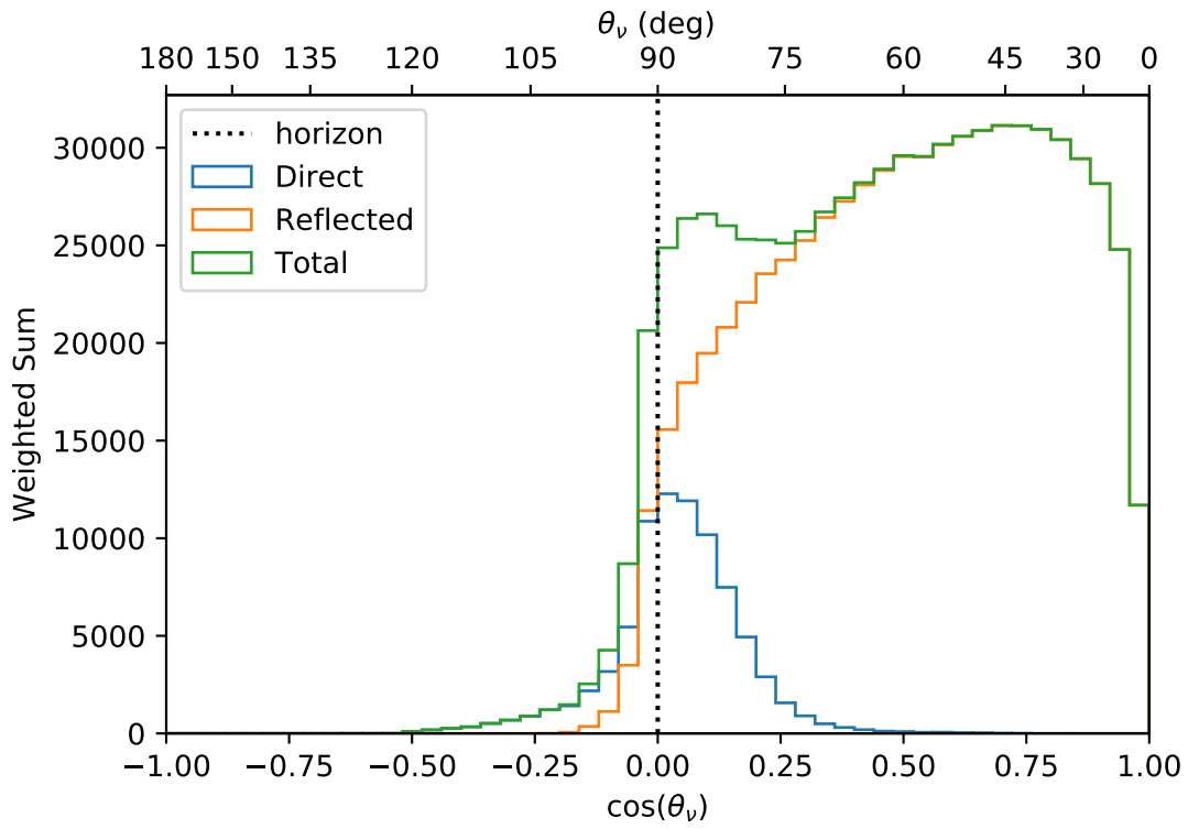
Figure 4.4: Neutrino arrival zenith, with 0^\circ representing a downward going neutrino. See Table 4.1 for simulation parameters.
