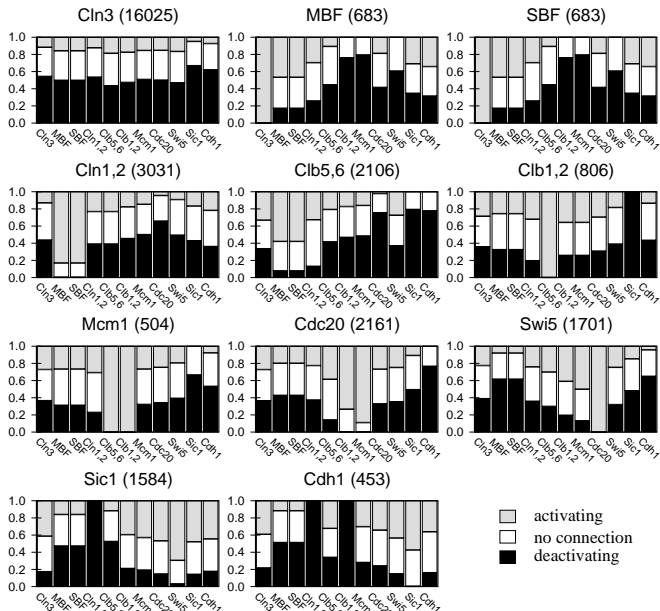
FIG. 2: Fractions of different types of inward connections to each node from all other nodes (including itself) that produce the cell-cycle process [see Table I]. Numbers in parenthesis are the number of connection combinations selected by our algorithm [see Methods].
