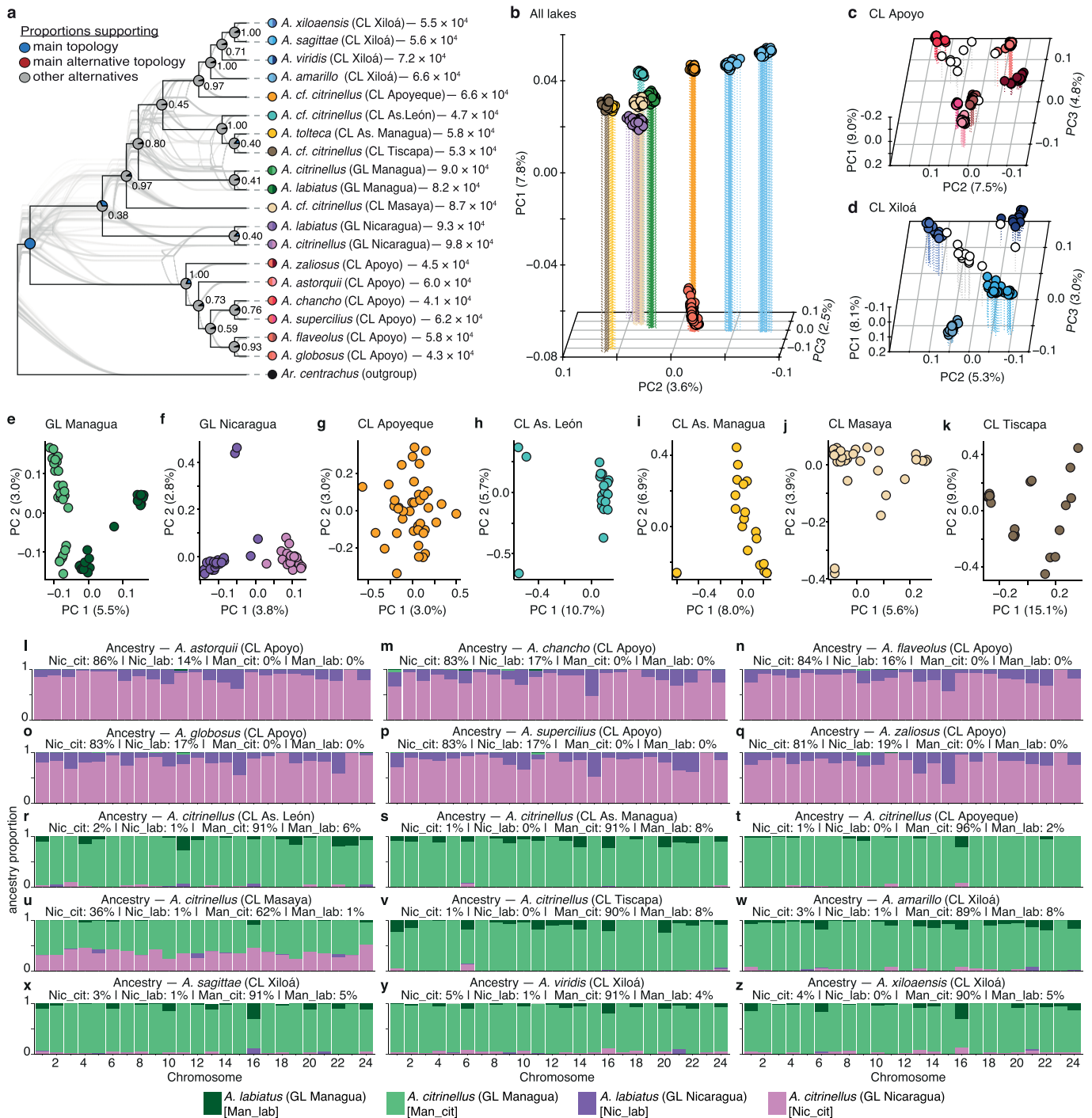
Extended Data Fig. 1 | Ancestry relationships in the Midas cichlid species complex. a , Inferred ASTRAL species tree, together with support, DensiTree visualization of bootstrapped species trees, and detected levels of gene tree – species tree discordance. Numbers after species names denote genome-wide \pi estimates, symbols before species names indicate colour code used in the rest of the figure (left half colour for lakes, right half colour for species). b–d , Clustering based on the first three dimensions of principal component analyses (PCAs) across all lakes ( b ), only CL Apoyo ( c ) and only CL Xiloá ( d ). Empty symbols indicate hybrids (that is, individuals with >25% admixed ancestry). e–k , Clustering based on the first two dimensions of principal component analyses of genomic variation in GLs Managua ( e ) and
