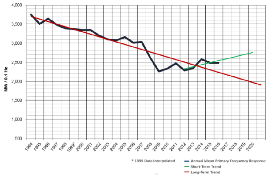
Figure 3. Decreasing total system inertia for the Eastern Interconnection 2
