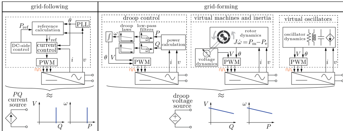
Figure 2. Functional diagrams of grid-following and grid-forming inverters. Grid-following inverters mimic current sources at their output terminals, whereas grid-forming inverters act like voltage sources whose output abides by droop laws.
