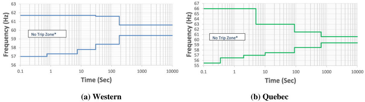
Fig. 5. Frequency No Trip Boundaries by Interconnection 4 .
