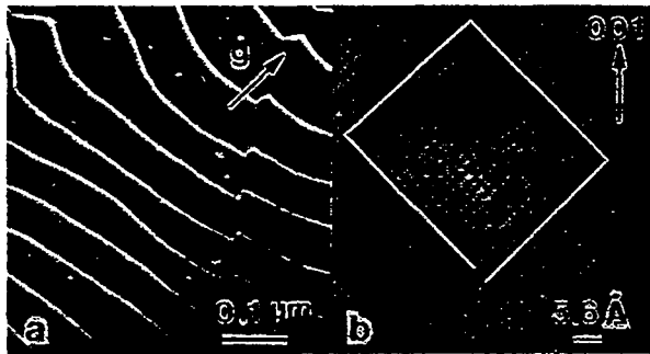
Fig. 4. TEM images of a sample annealed at 800°C for 30 min. (a) A plan view image with g=[040] . (b) A cross section image viewed along the [100] direction showing that the dislocation has a Burgers vector b=\frac{a}{2}[01\bar{1}] , as indicated on the Burgers circuit.
