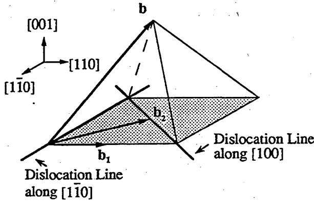
Fig. 5. When a dislocation with Burgers vector b = \frac{a}{2}[011] is bent from the [1\bar{1}0] toward the [100] direction, the edge component of the Burger vector in (001) interfacial plane changes from b_1 = \frac{a}{4}[110] to b_2 = \frac{a}{2}[010] .
