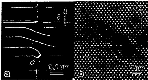
Fig. 2. TEM images of a sample annealed at 600^\circ\text{C} for 30 min. (a) A plan view image with \mathbf{g}=[220] . A segment of dislocation with \mathbf{b} = \frac{a}{2}[110] was observed between two nodes (marked by arrow). (b) A cross section lattice image viewed along a \langle 110 \rangle direction.
