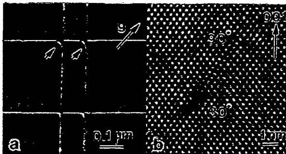
Fig. 1.(a) A plan view TEM image of misfit dislocations in an as-grown specimen with the diffraction vector g=[400] . Note the crossing reactions at nodes, as indicated by arrows. (b) A cross section lattice image viewed along a \langle 110 \rangle direction.
