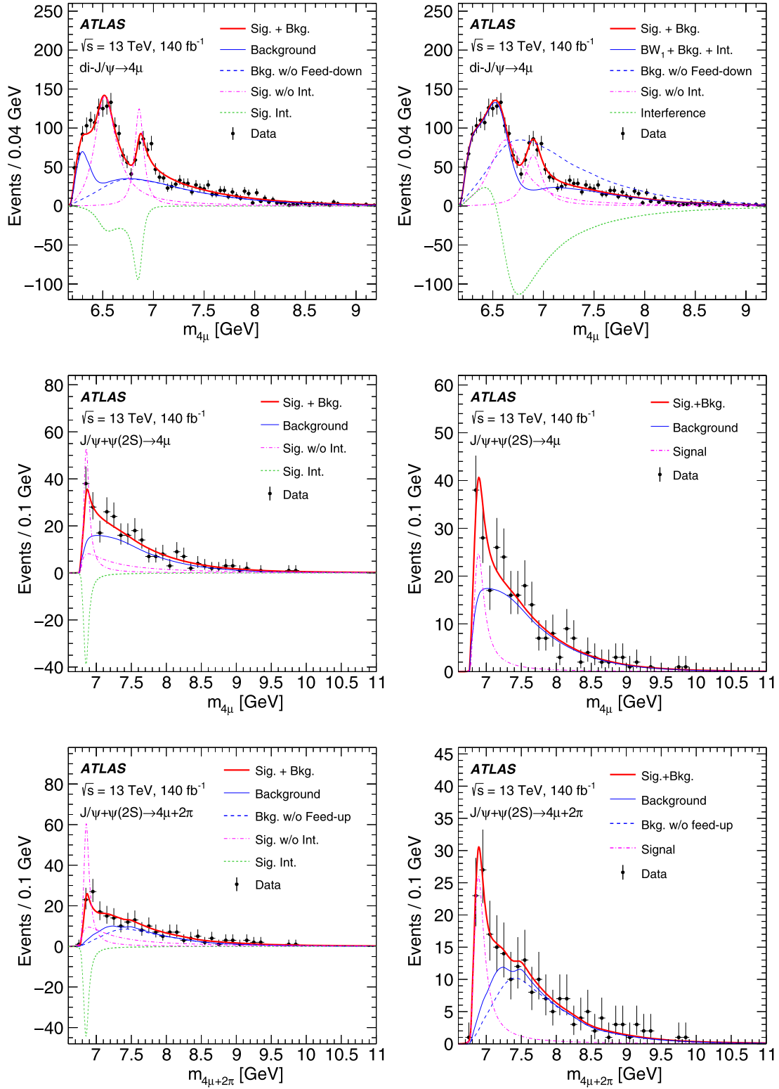
FIG. 5. Fits to the di- J/\psi and J/\psi + \psi(2S) mass spectra in the SRs for models A (left) and B (right). For each model, the di- J/\psi spectrum (top) and the J/\psi + \psi(2S) spectra in the 4\mu (middle) and 4\mu + 2\pi (bottom) channels are shown. The purple dot-dashed lines indicate the components of individual resonances, while the green short-dashed ones represent the interferences. Note that no interference is present in the J/\psi + \psi(2S) channels for model B since X(6900) is standalone.
