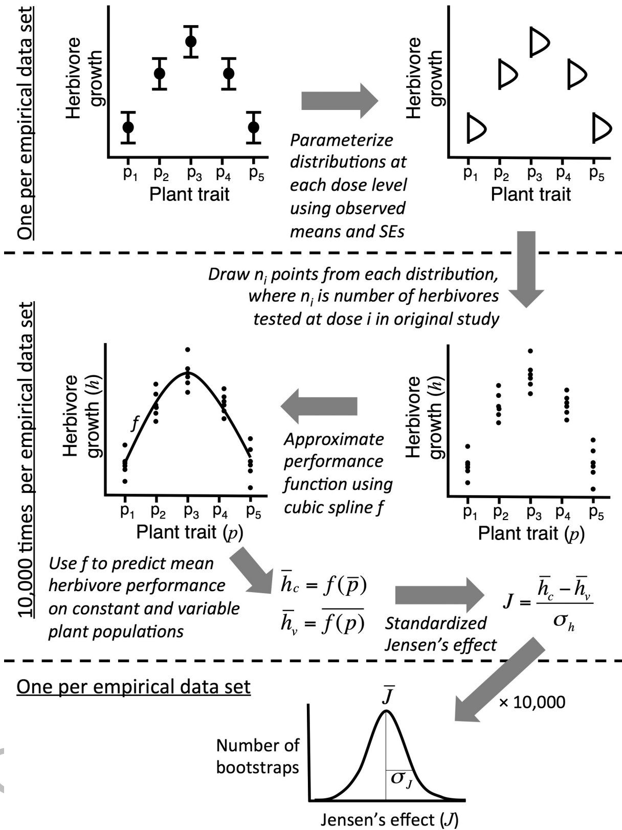
Extended Data Figure 2 | Visual representation of quantitative methods. This diagram summarizes the bootstrapping algorithm used to calculate a distribution of Jensen's effects for each empirical data set for herbivore growth. For more details and for differences in methods between growth and survival see Methods and Supplementary Methods.
