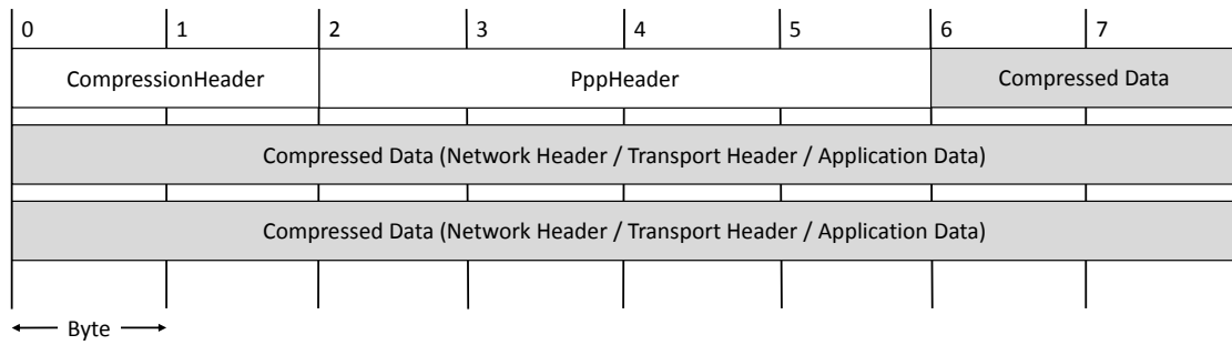
Figure A.1: Header format of the compressed packet using our ns-3 module.
