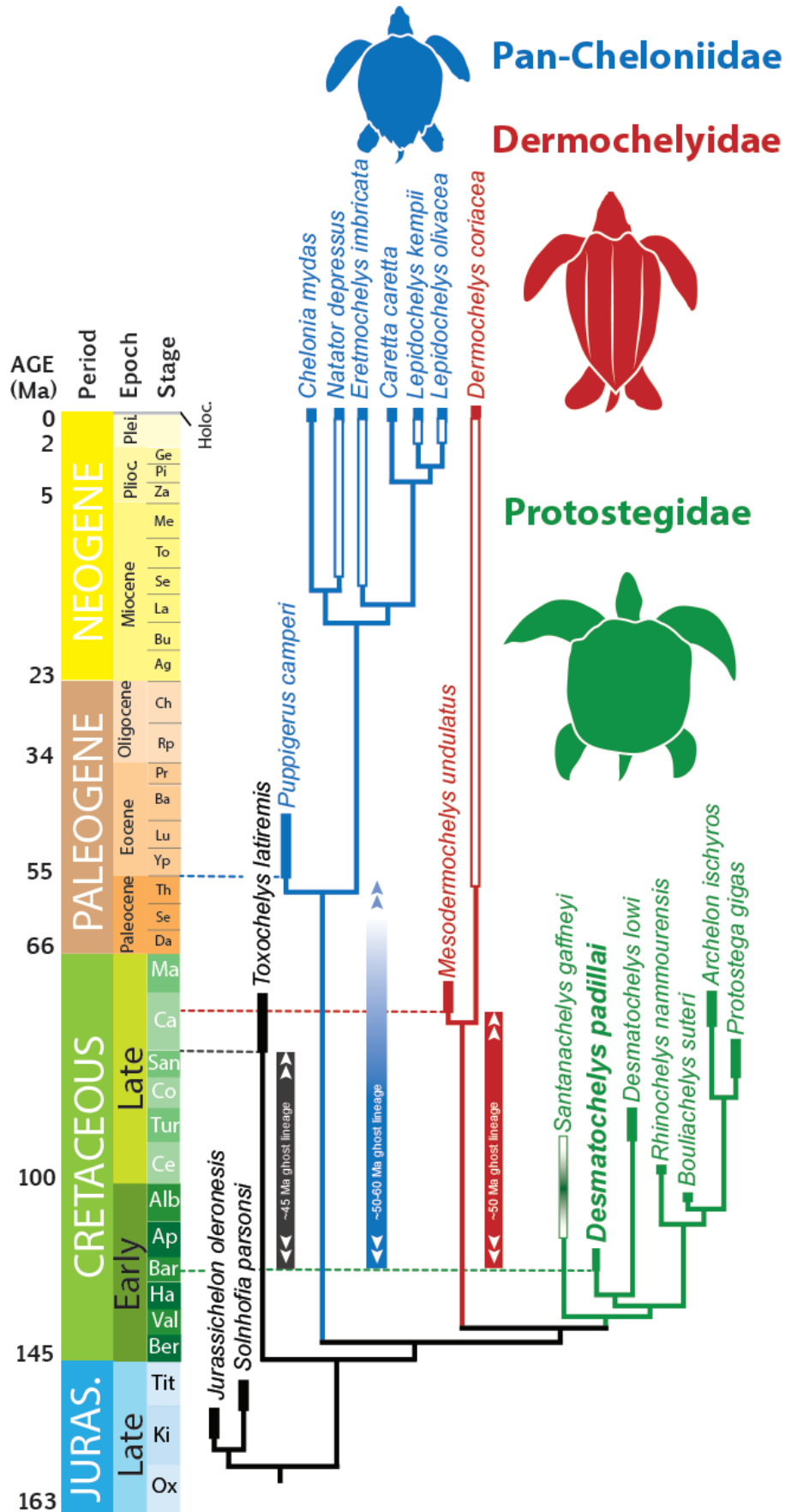
Figure 12. Chronostratigraphic distribution of Pan-Chelonidoidea clade matching the topology presented in Figure 11. Solid square-rectangles at the tip branches are based on the fossil occurrences. White rectangles represent fossils that show the age of the stem lineages. The data for these are from Parham and Pynson (2010) with a correction to the age of crown group cheloniids to Zancian instead of Serravalian. Note that some taxon ranges are long due to stratigraphic uncertainty and should not be interpreted as illustrating a continuous fossil record. For S. gaffneyi we use a gradient fill to emphasize this. Taxon ranges for fossil occurrences were taken from literature as follows, starting from the left: Jurassichelon oleronesis from Pérez-García (2015), Solnhofia parsonsi from Joyce (2000), Toxochelys latiremis from Hirayama (1997), see also Joyce et al. (2013), Puppigerus camperi from Moody (1974), Mesodermochelys undulatus from Hirayama and Chitoku (1996) and Hirayama et al. (2006), Santanachelys gaffneyi from Hirayama (1998) see also Martill (2007) and Joyce et al. (2013), Desmatochelys padillai from this study, Desmatochelys lowi from Elliot et al. (1997) and Hirayama (1997), Rhinochelys nammourensis from Tong et al. (2006), Archelon ischyros from Hirayama (1997), and Protostega gigas from Hirayama (1997). Extensive ghost lineages are shown for three taxa ( Toxochelys , Pan-Cheloniidae, and Dermochelyidae) with the upper range for Pan-Cheloniidae shown as uncertain because of Maastrichtian and Paleocene taxa that need to be integrated into phylogenetic analyses (see Parham et al. 2014).
