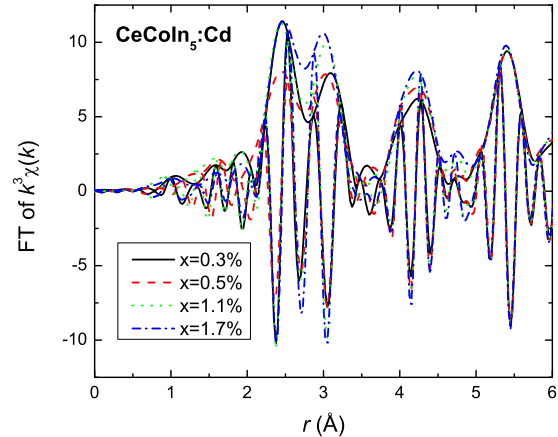
FIG. 6: (Color online) FT of k^3(\chi(k)) data for all measured Cd-substituted samples. Note changes in local structure. Despite these changes, no clear trends with x are deduced from the fit results.
