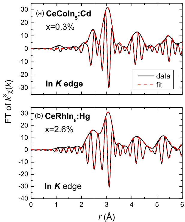
FIG. 4: (Color online) Representative fits to Fourier transform (FT) of k^3\chi(k) In K -edge data. All transforms are between 2.5 - 16.0 \text{ \AA}^{-1} after Gaussian narrowing by 0.3 \text{ \AA}^{-1} unless otherwise noted. The outer envelope is the modulus, and the oscillating line is the real part of the complex transform. The difference in Co and Rh backscattering is demonstrated by the large difference in the first peak near 2.5 \text{ \AA} , due primarily to (a) In(2)-Co or (b) In(2)-Rh scattering paths.
