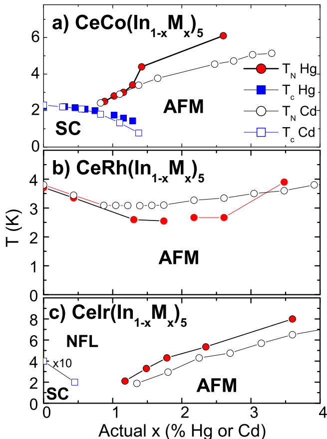
FIG. 2: (Color online) Phase diagrams of Cd- and Hg-substituted Ce T In _5 . The reported substituent concentrations of Cd-substituted samples are estimated from microprobe measurements of the Hg-substituted samples. See Sec. II for details.
