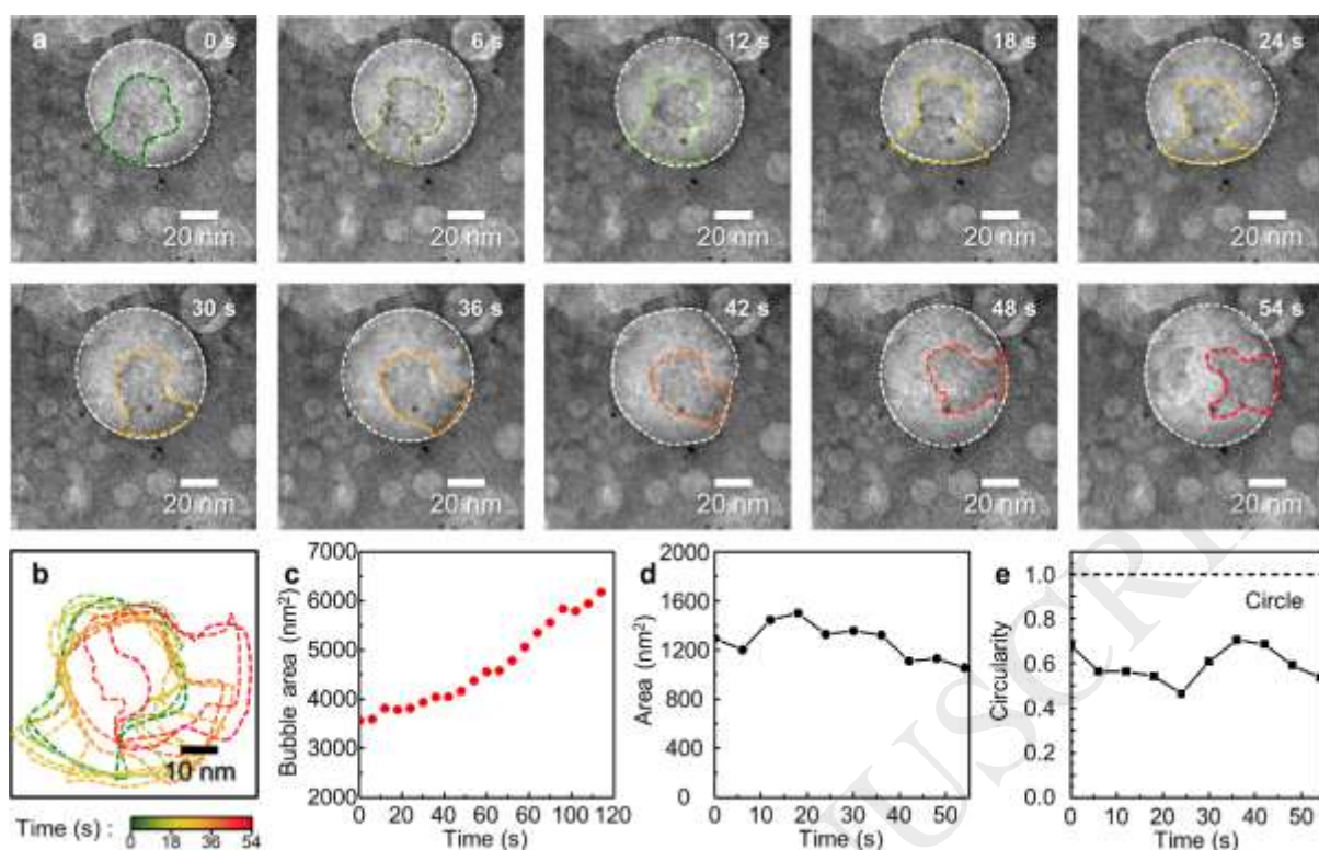
Figure 2. Deformation of the liquid under the strong electron beam. (a) A time-series of in situ TEM images showing the liquid deformation under the strong electron beam ( 400 \text{ e}^-/\text{\AA}^2 \cdot \text{s} ). The colored and the white dashed lines highlight the deformed liquid and gas bubbles. The images are extracted from Movie S4. (b) A contour plot of the liquid boundaries. (c) Plot of the bubble area acquired from the white dashed lines as a function of the measurement time. (d,e) Plots showing the area (d) and the circularity (e) of the deformed liquid part (highlighted by the color dashed lines in panel a) as a function of time.
