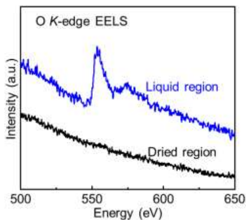
Figure S5. Electron energy loss spectroscopy (EELS) spectra of liquid and dried parts of the graphene liquid cell used in this study.
