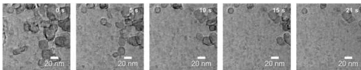
Figure S3. In-situ TEM images showing dynamics of NaCl in the dried area of graphene liquid cells. The images are extracted from Movie S3.
