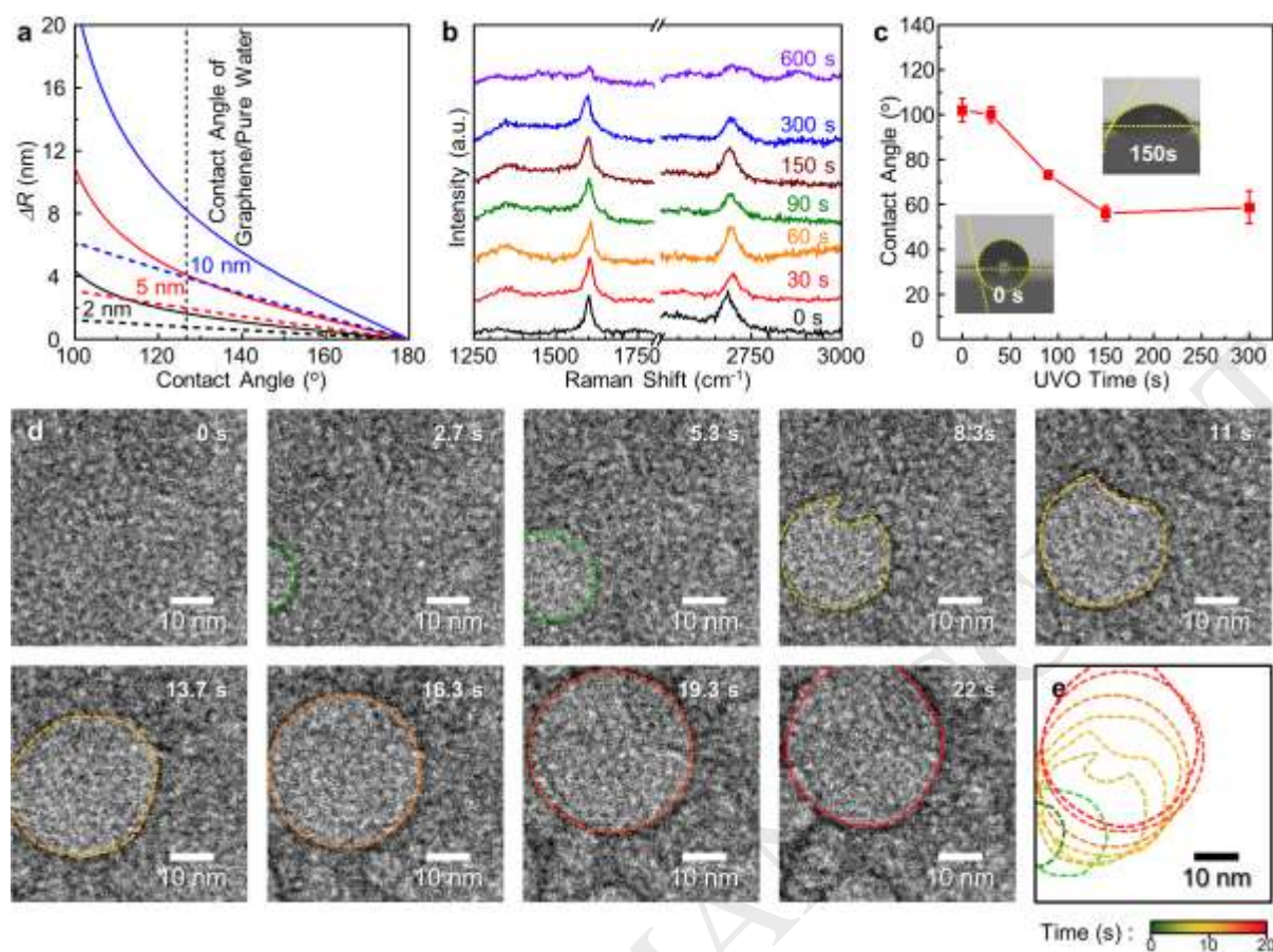
Figure 4. Experiment with a hydrophilic graphene liquid cell for comparison. (a) The calculated step movement lengths of nanodroplets with different droplet radii (2, 5, and 10 nm) according to the contact angle. The solid and dashed lines represent the cylinder model and the hemisphere model. (b) Raman spectra of graphene according to the UVO treatment time. (c) Macroscopic contact angles of pure water on the graphene-coated grids as a function of the UVO treatment time. The insets display representative photograph images acquired from non-treated and UVO treated (150 s) graphene-coated grids. (d) A time-series of in situ TEM images showing dynamic behaviors of the liquid in the graphene liquid cell after surface treatment. The images are extracted from Movie S6. (e) A contour plot of the liquid-gas boundaries.
