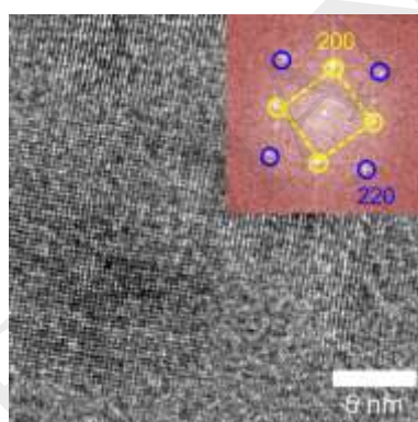
Figure S4. A representative high-resolution TEM image of NaCl observed in the dried part of the graphene liquid cells. The inset shows FFT of the image.
