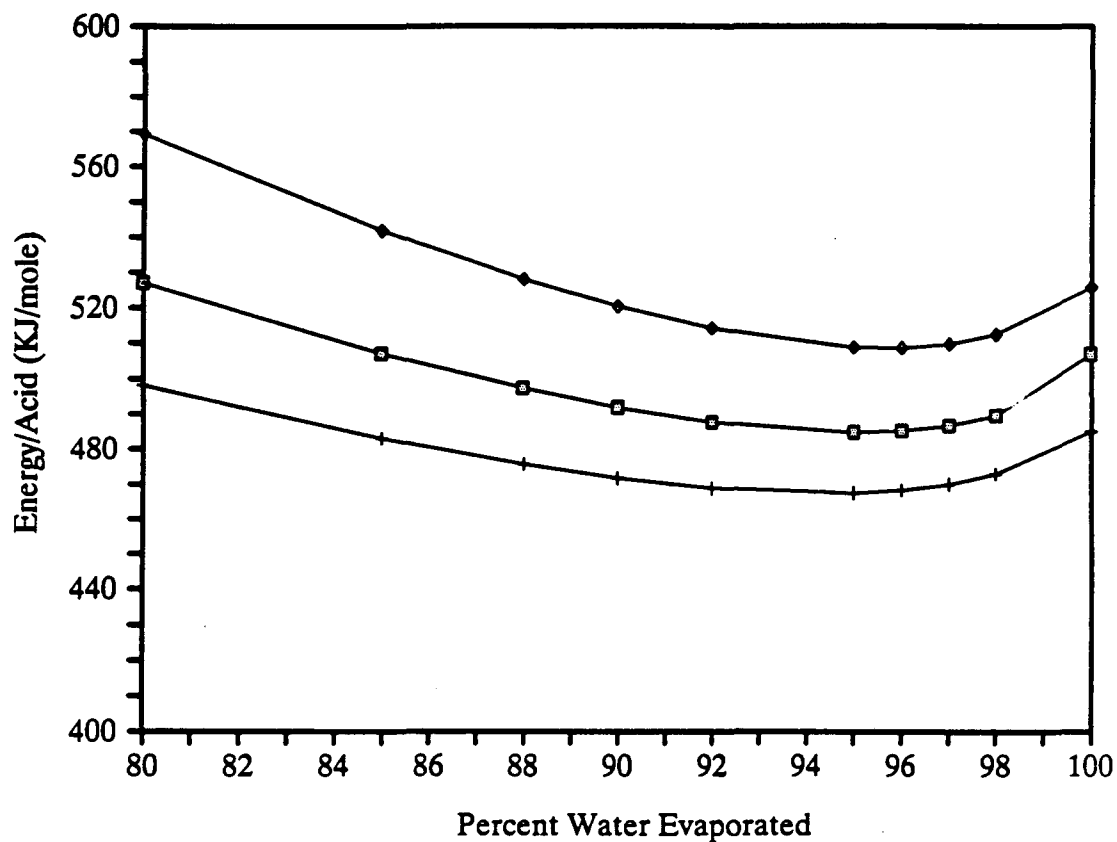
Figure 7.10 Energy required per mole of acid recovered for three different acid concentrations in the aqueous feed for the adipic acid - cyclohexanone system with a two stage evaporation process.
