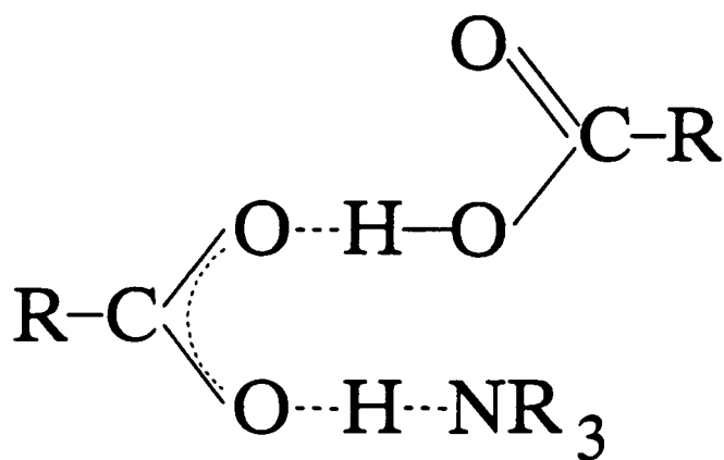
Figure A.4 The formation of a hydrogen bond between the -OH of the second acid to the conjugated CO of the complexed acid explains the overloading phenomena found experimentally in methylisobutylketone.
