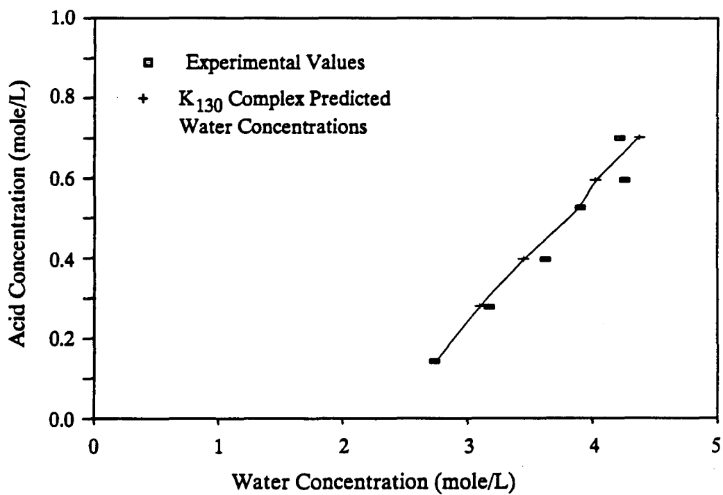
Figure 5.5 Succinic acid - methylcyclohexanone liquid - liquid equilibrium at 45C with predicted water concentration from complexation model.
