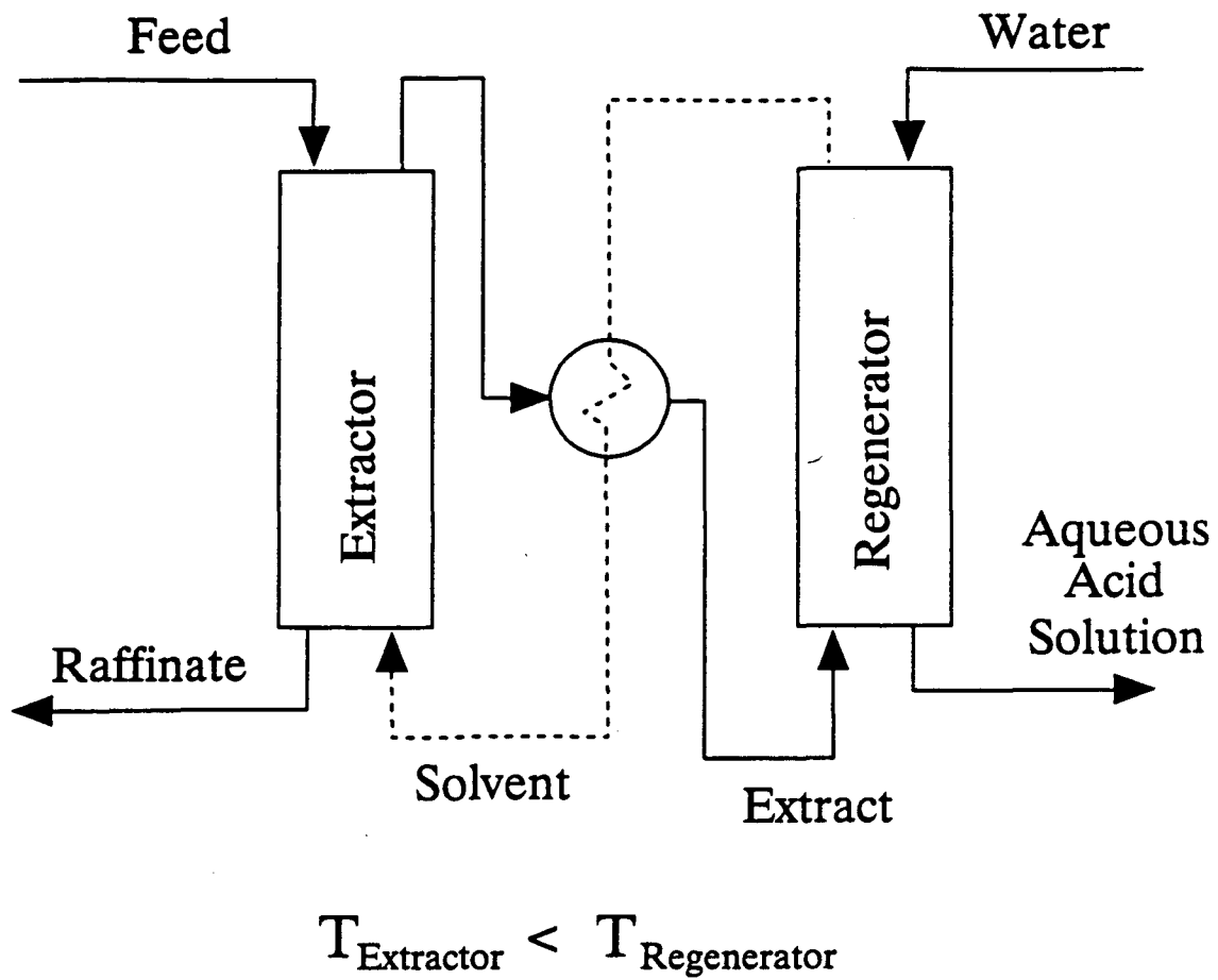
Figure 1.1 Temperature swing process flowsheet
